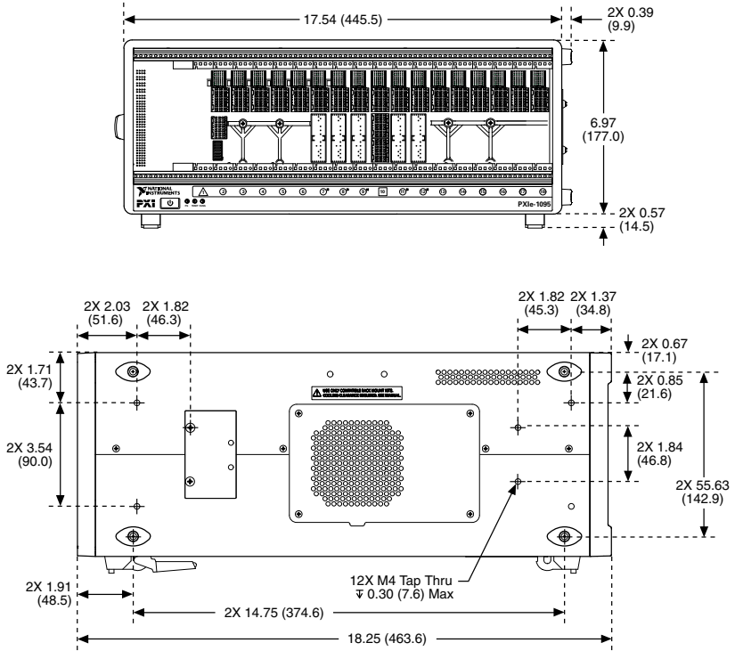
Figure 1. PXle-1095 Chassis Dimensions (Front and Side)
