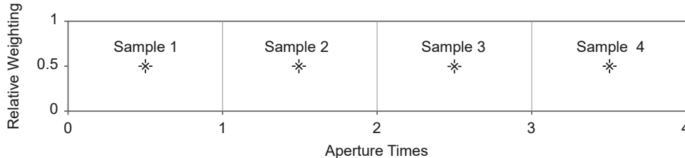
Figure 19. Normal Noise Rejection
