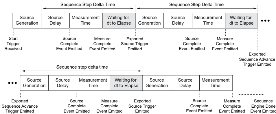
Figure 22. Sequence Step Delta Time in NI-DCPower Sequences
