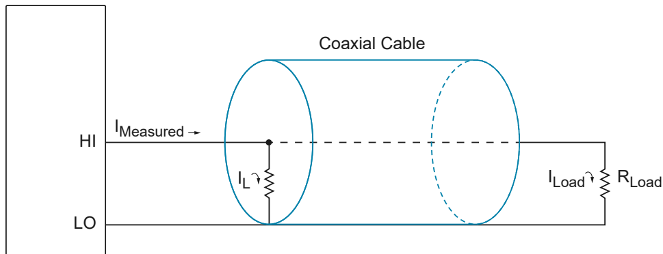
Figure 14. Leakage without Guarding ( I_{Measured} = I_{Load} + I_L )
