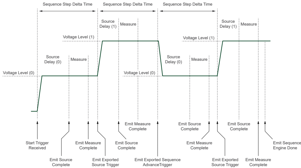
Figure 21. Sequence Step Delta Time Source Model
