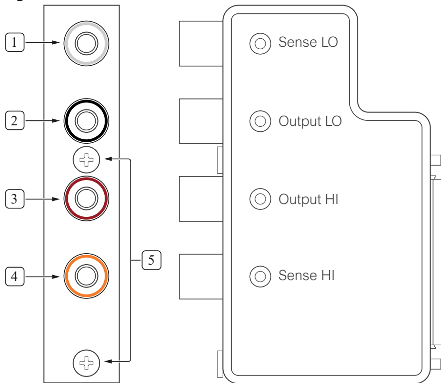
Figure 10. SA-413B Front Panel
