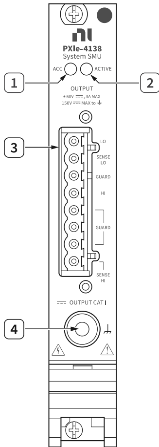
Figure 3. PXle-4138 Front Panel
