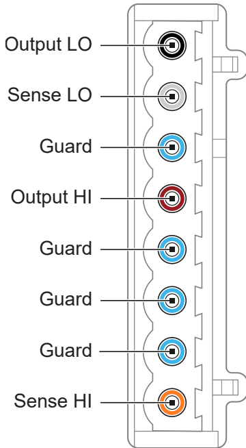
Figure 4. PXle-4138 Connector Pinout
