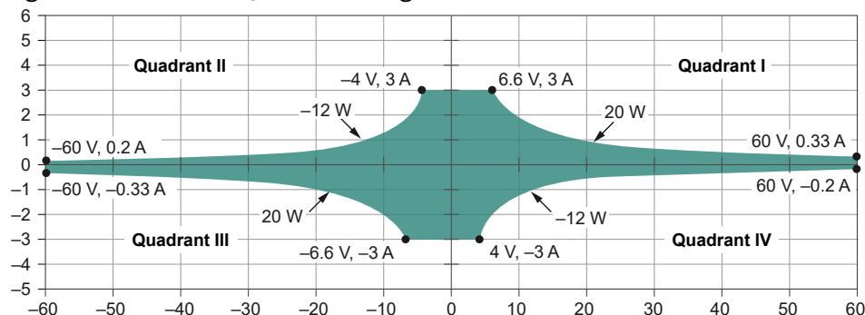
Figure 1. PXIe-4138 Quadrant Diagram
