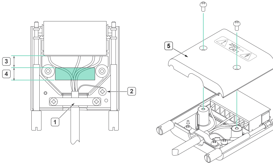
Figure 7. PXle-4138 Output Connector Preparation
