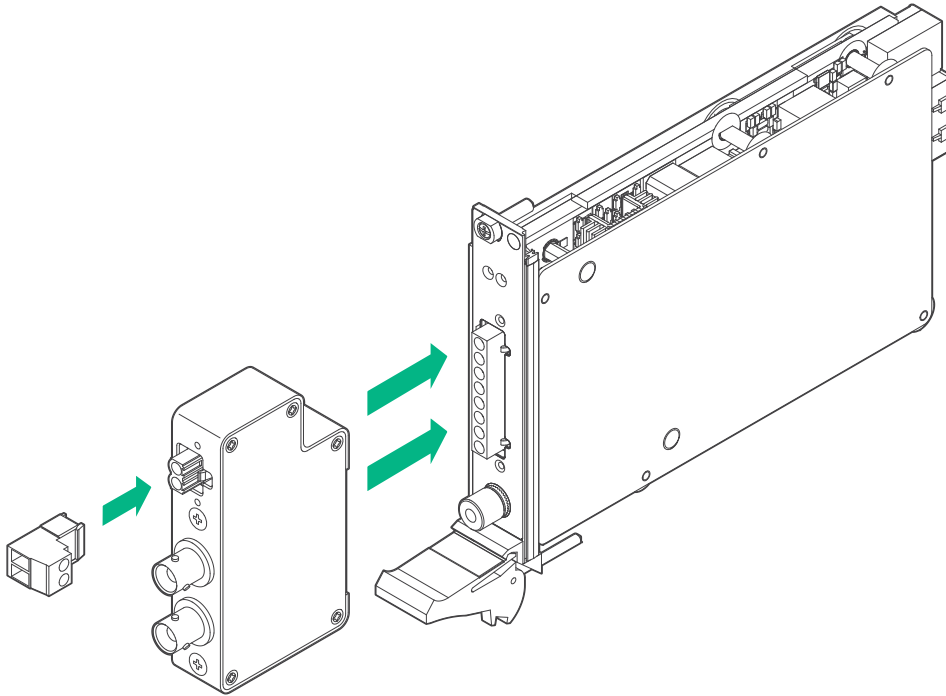
Figure 8. SA-413T Installation with a PXle-4138
