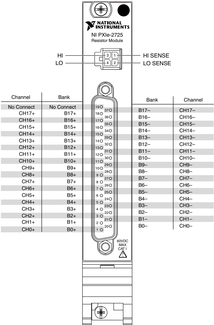
Figure 3. NI 2725 Connector Pinout
