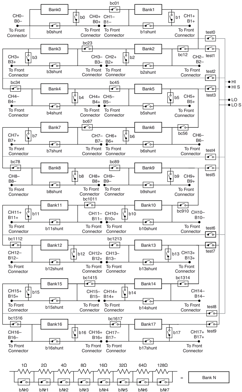
Figure 4. NI 2725 Power-on State
