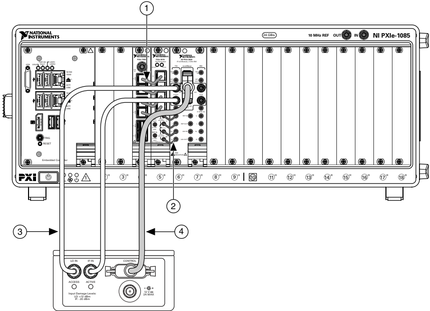
Figure 32. Connecting the mmRH-3647 to the Unidirectional SISO (Baseband and IF) TX Chassis
