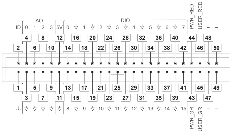
Figure 4. USB-6423 (OEM) AO/DIO Connector Pinout
