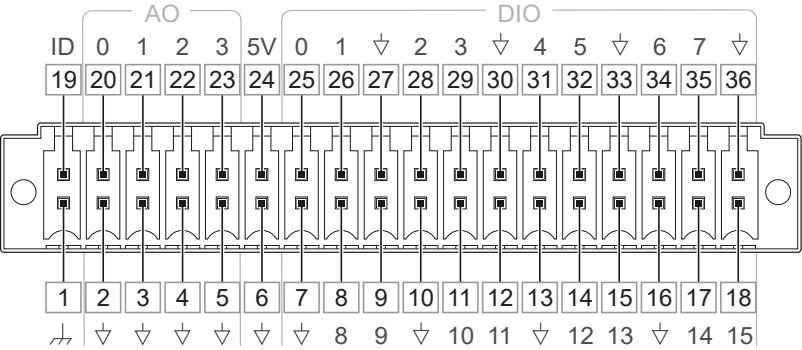
Figure 2. USB-6423 AO/DIO Connector Pinout
