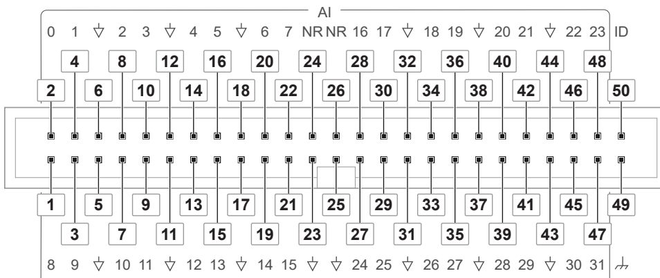
Figure 3. USB-6423 (OEM) AI Connector Pinout
