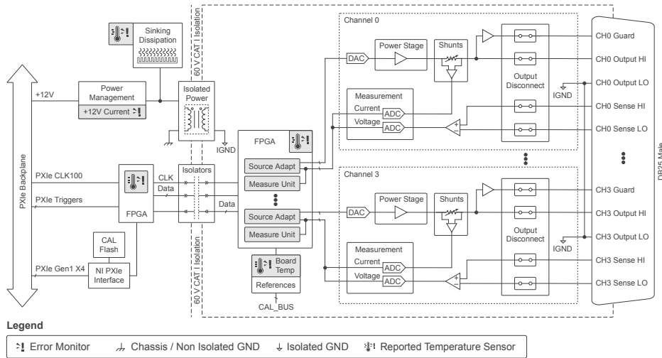
Figure 3. PXIe-4147 Channel-Level Block Diagram
