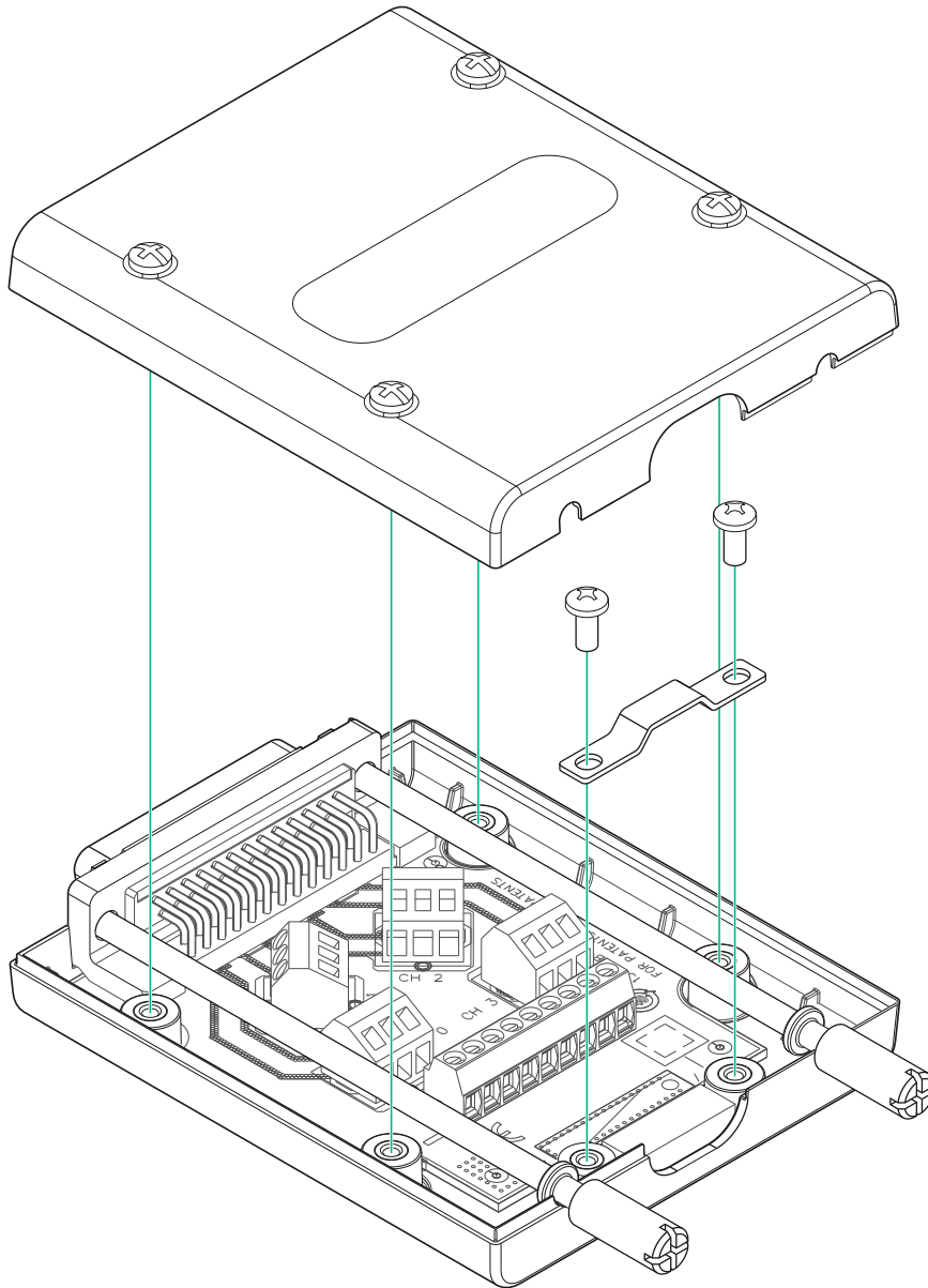
Figure 8. Disassembled TB-414X
