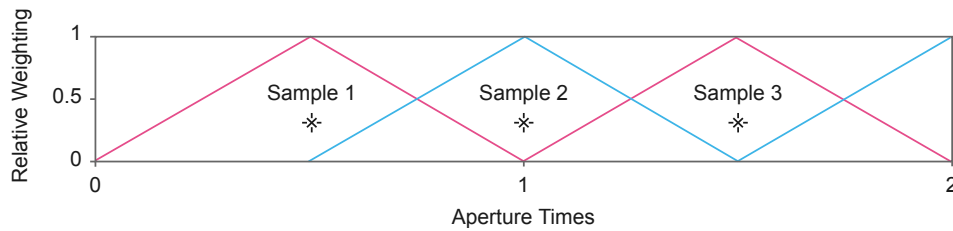
Figure 20. Second-Order Noise Rejection
