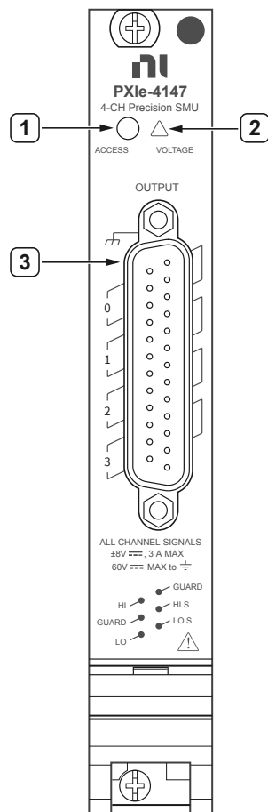
Figure 4. PXIe-4147 Front Panel
