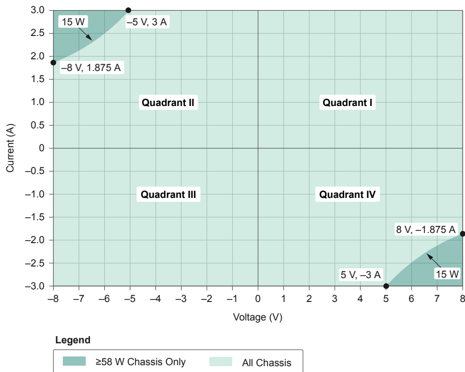
Figure 1. PXIe-4147 Quadrant Diagram
