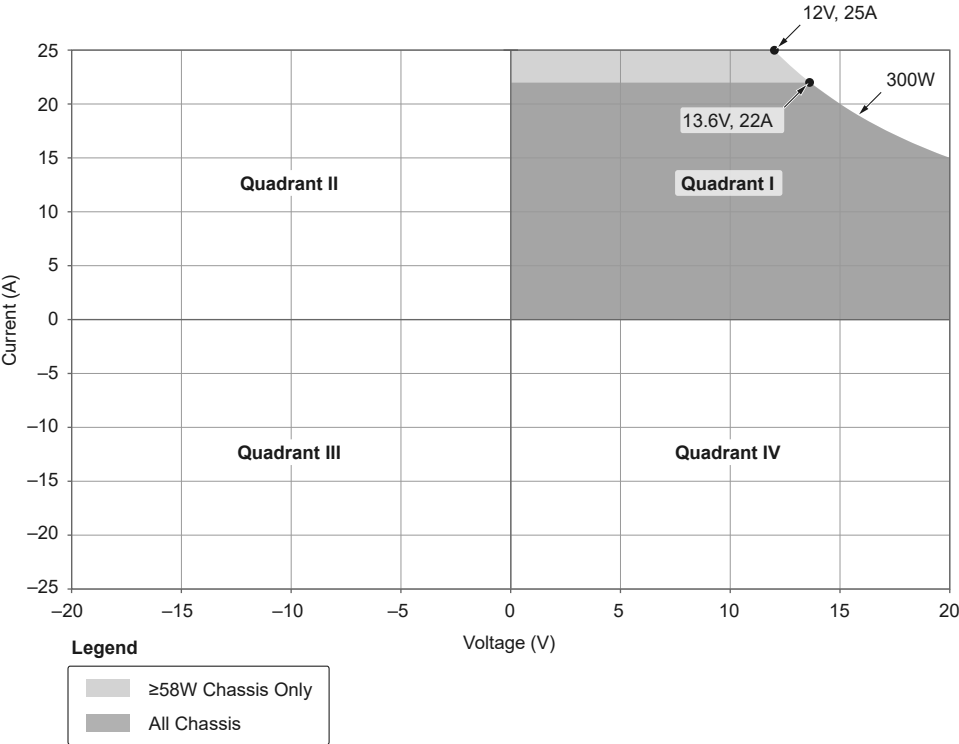
Figure 5. PXle-4151 Quadrant Diagram, T ambient >40 °C
