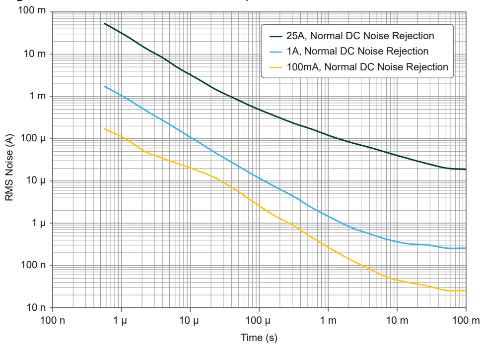
Figure 7. Current RMS Noise Versus Aperture Time, Nominal
