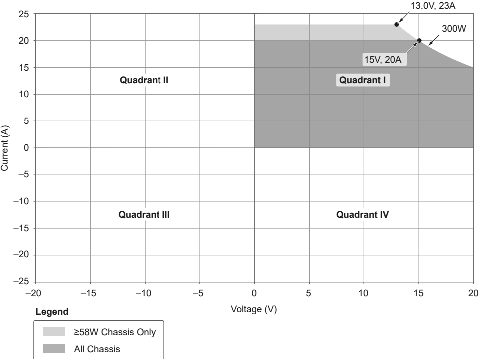
Figure 5. PXle-4151 Quadrant Diagram, T ambient >40 °C
