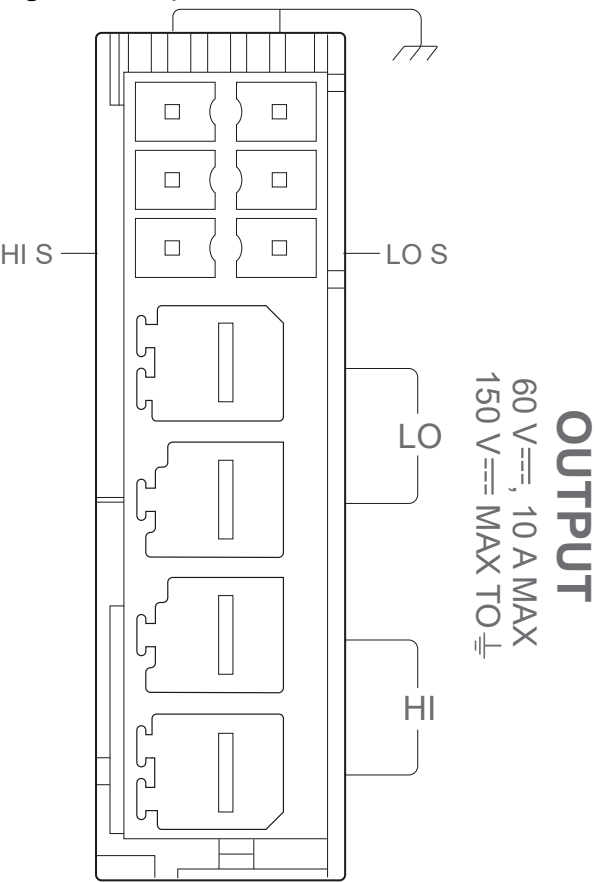
Figure 1. Output Connector Pinout
