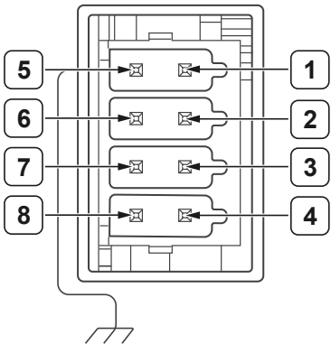
Figure 2. AUX I/O Connector Pinout
