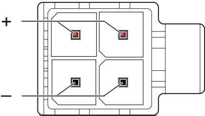
Figure 3. AUX Power In Connector Pins
