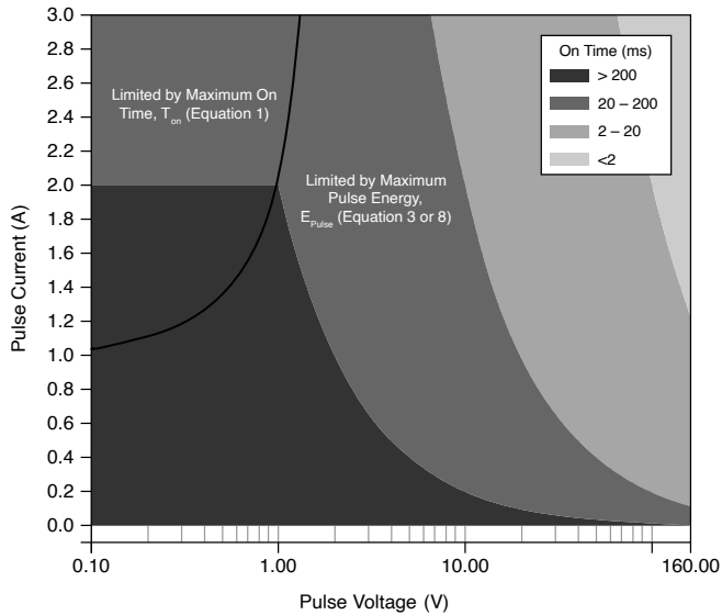
Figure 9. Pulse On-time vs Pulse Current and Pulse Voltage
