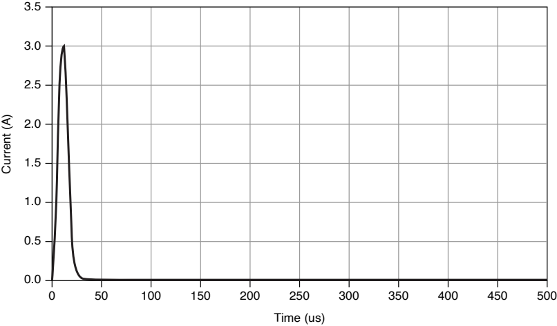
Figure 14. 10 \mu s Pulse Output with Load, Custom Transient Response
