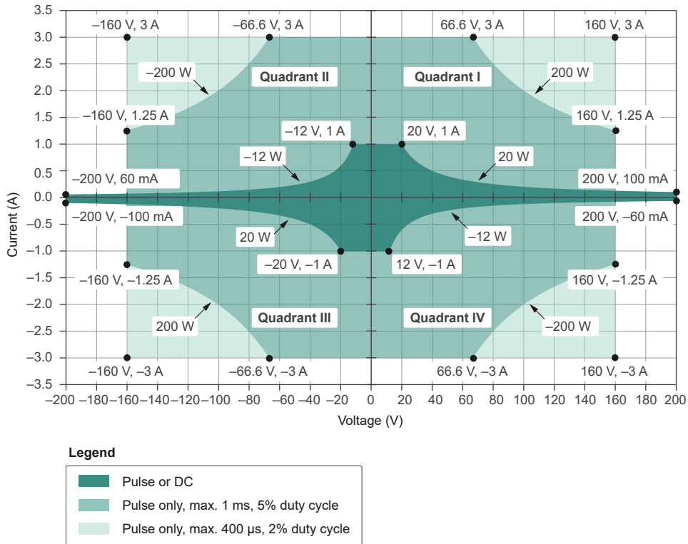
Figure 2. Quadrant Diagram for PXle-4135 (20W)
