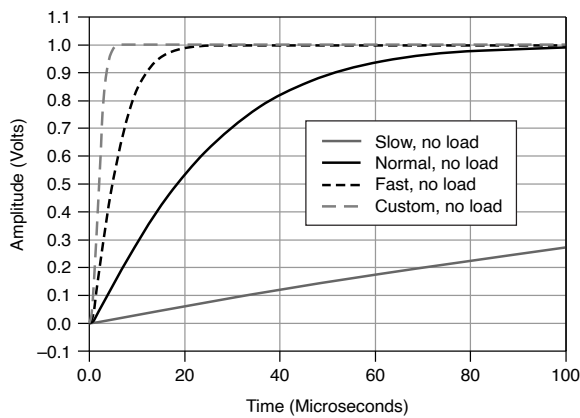
Figure 11. 1 mA Range, No Load Step Response, Nominal
