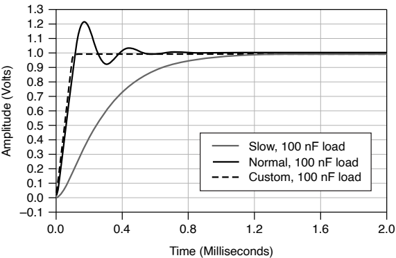
Figure 12. 1 mA Range, 100 nF Load Step Response, Nominal
