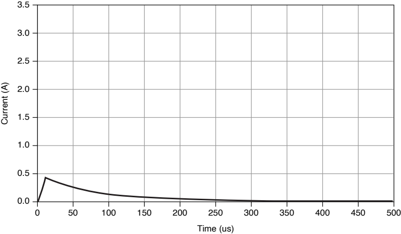
Figure 13. 10 \mu s Pulse Output with Load, Fast Transient Response
