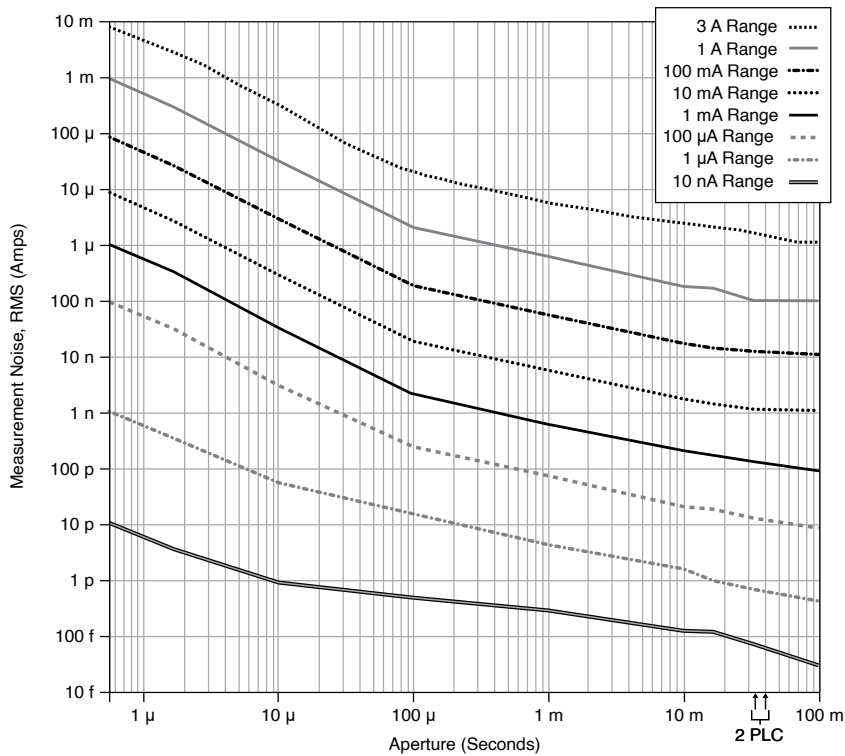
Figure 4. Current Measurement Noise vs. Measurement Aperture, Nominal
