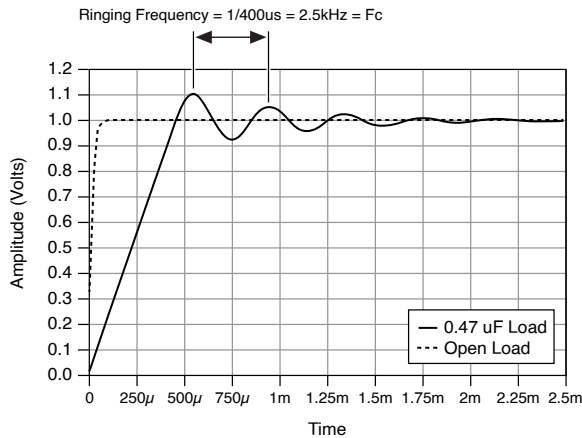
Figure 15. Example of Ringing Frequency
