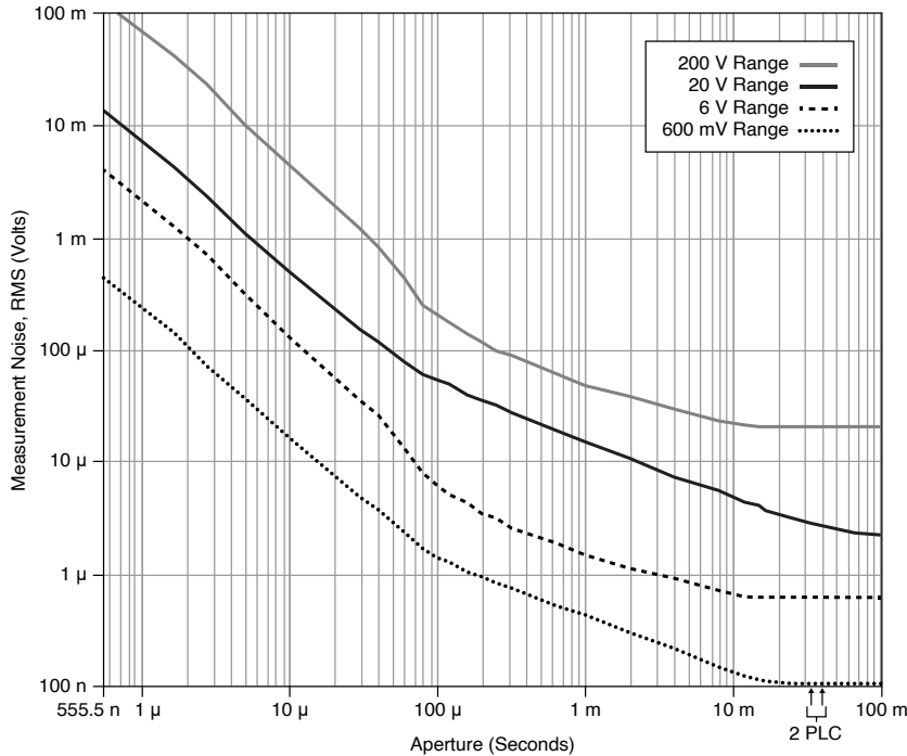
Figure 3. Voltage Measurement Noise vs. Measurement Aperture, Nominal
