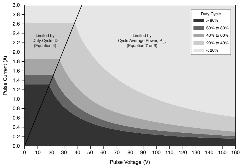
Figure 10. Duty Cycle vs Pulse Current and Pulse Voltage
