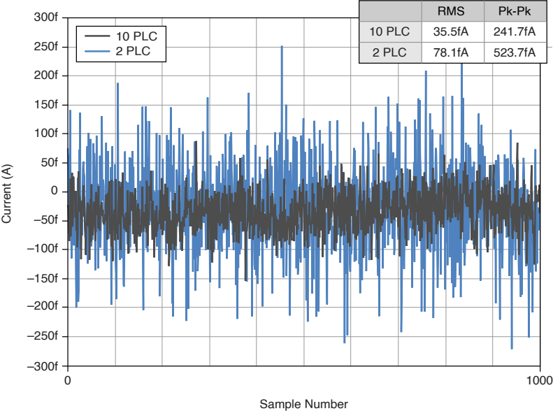
Figure 6. Measurement Noise, 10 nA Range, 1 GΩ Load, 9 V, 3 m Cables, Nominal
