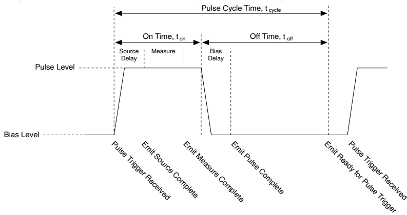
Figure 8. Definition of Pulsing Terminology
