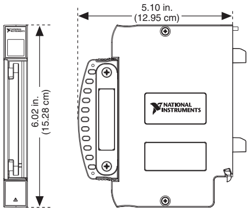
Figure 10. TB-4300/B/C Dimensions
