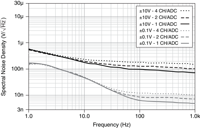
Figure 15. 2 kS/s Spectral Noise Density (Multichannel per ADC)
