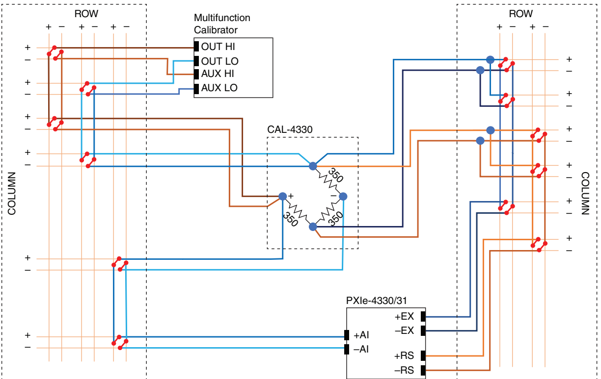
Figure 12. Gain Accuracy Verification
