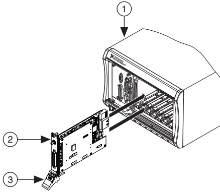
Figure 2. Sliding the PXle-4480/4481 into the Chassis
