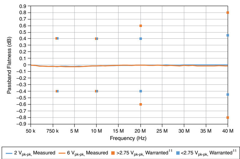
Figure 1. Passband Flatness
