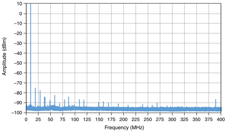
Figure 9. 10 MHz Single-Tone Spectrum 25 , Measured
