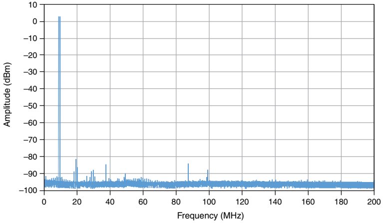
Figure 10. 9.5 MHz and 10.5 MHz Dual-Tone Spectrum 26 , Measured
