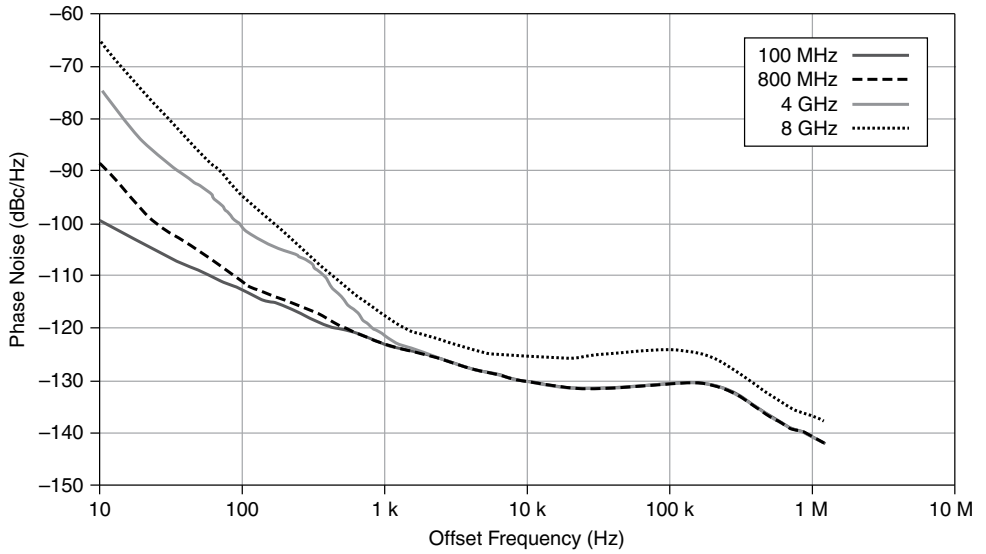
Figure 2. Nominal Phase Noise at 100 MHz, 800 MHz, 4 GHz, and 8 GHz 7, 8
