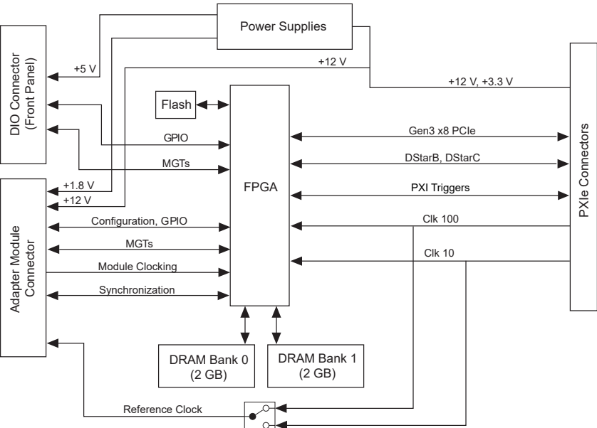
Figure 12. PXle-5774 Block Diagram
