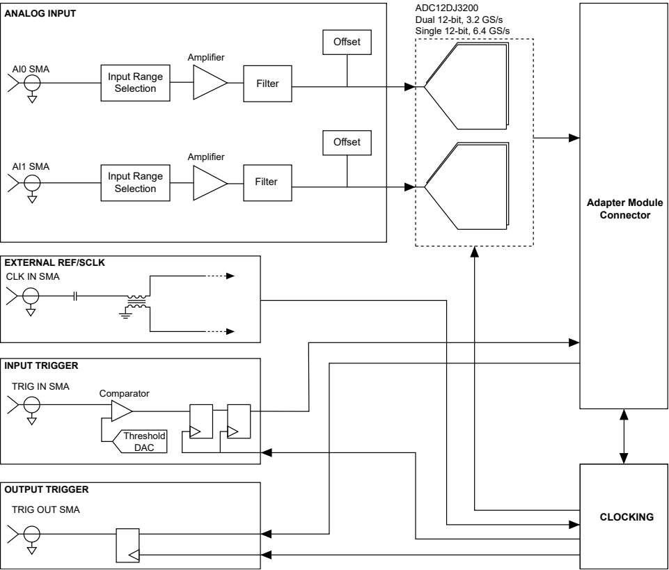
Figure 12. PXle-5774 Block Diagram
