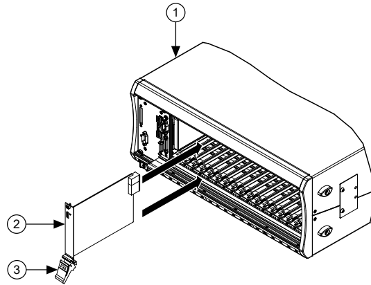
Figure 7. Module Installation
