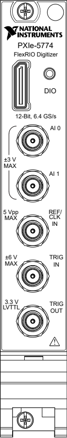
Figure 10. PXIe-5774 Front Panel
