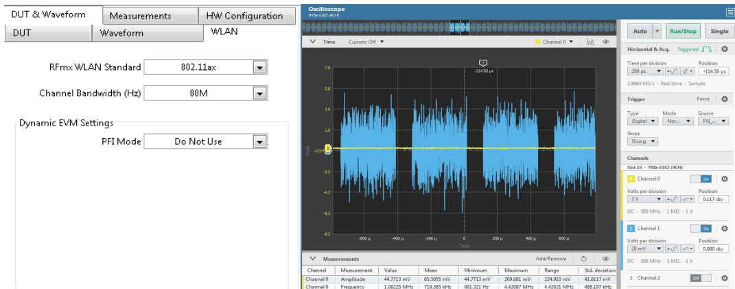
Figure 8: Scope Trace of RF and Enable Pulse without PFI
