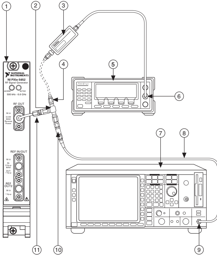
Figure 1. Splitter Characterization Setup
