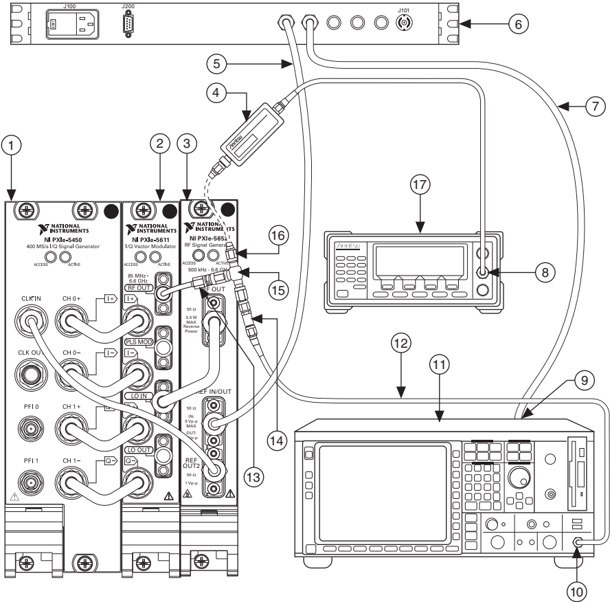
Figure 2. Connecting Hardware to Verify Output Power Level Accuracy
