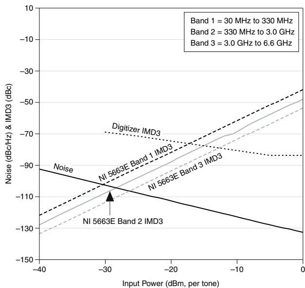
Figure 4. PXIe-5663E Nominal Dynamic Range, 0 dBm Reference Level
