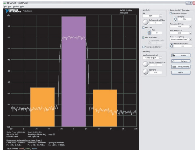
Figure 5. ACP Measurement of a QPSK Signal
