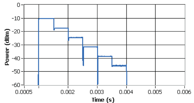
Figure 3. Deterministic 500 \mu s Power Steps Using the NI PXIe-5663E and RF List Mode
