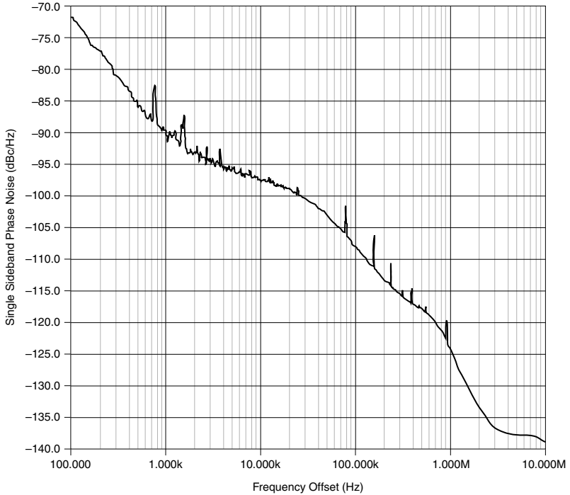
Figure 3. Typical Phase Noise at 5.8 GHz
