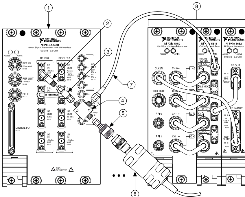
Figure 18. Input Frequency Response Verification Cabling Diagram
