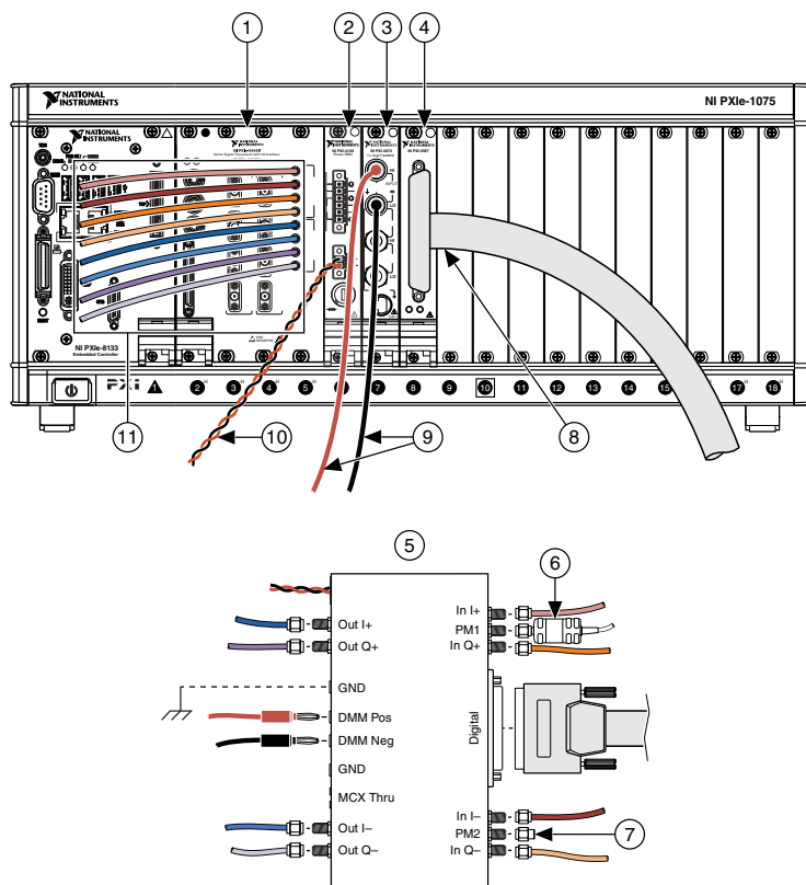
Figure 2. Recommended PXIe-5645 I/Q Calibration System
