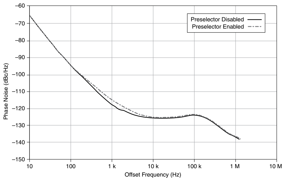
Figure 3. PXle-5665 14 GHz VSA Nominal Phase Noise at 8 GHz 8
