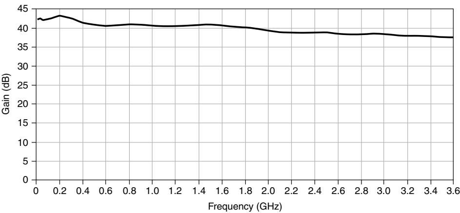
Figure 16. PXIe-5603 Typical Maximum Conversion Gain (Center Frequency <3.6 GHz)
