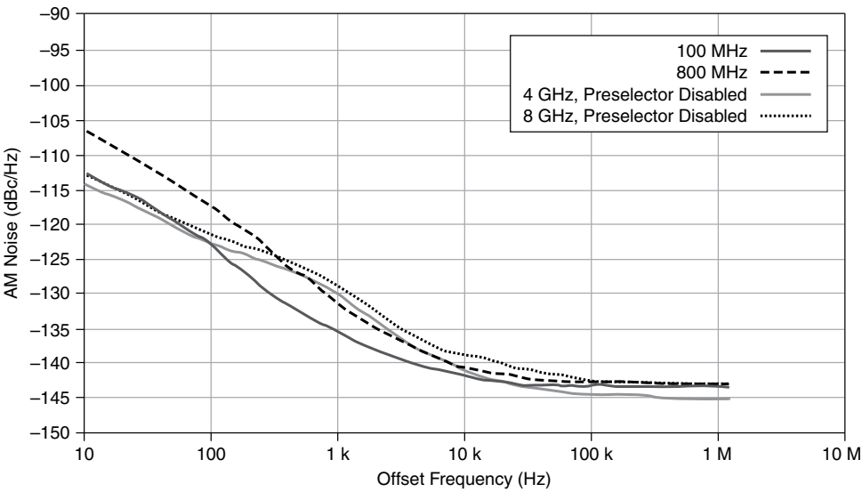
Figure 4. Nominal AM Noise for Carrier Frequencies of 100 MHz, 800 MHz, 4 GHz, and 8 GHz (Nominal, Spurs Not Shown) 9
