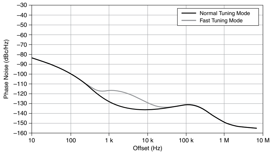
Figure 13. LO1 Phase Noise Measured Performance Comparison, Normal Tuning Versus Fast Tuning Speed 41
