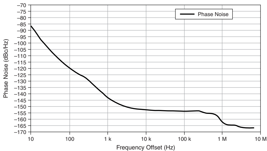
Figure 15. LO3 Phase Noise 45
