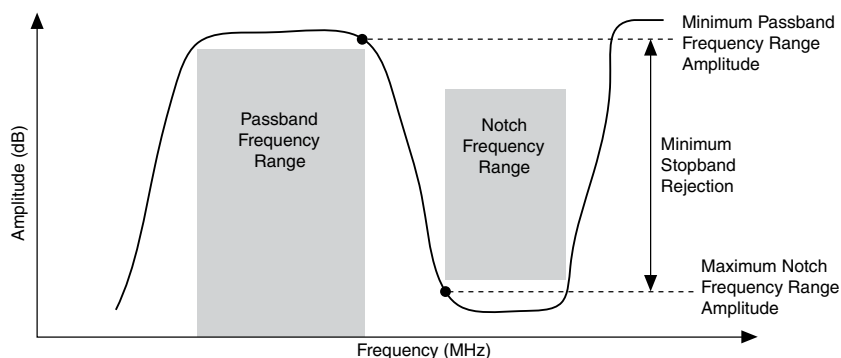
Figure 3. PXIe-5693 Notch Filter Frequency Range Definition
