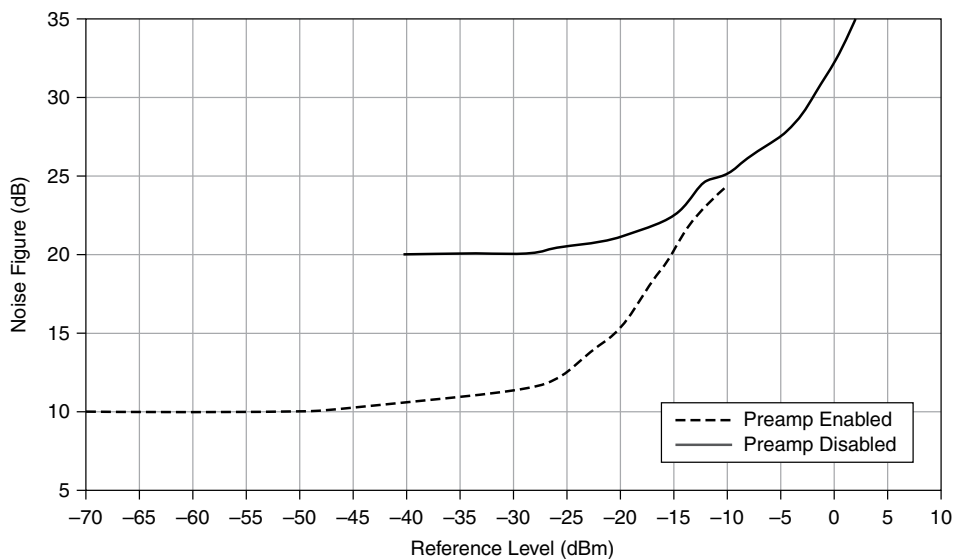
Figure 4. Noise Figure versus Reference Level (Nominal) 40
