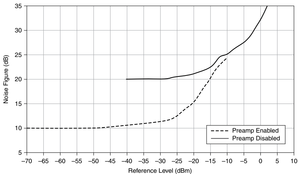
Figure 4. Noise Figure versus Reference Level (Nominal) 42
