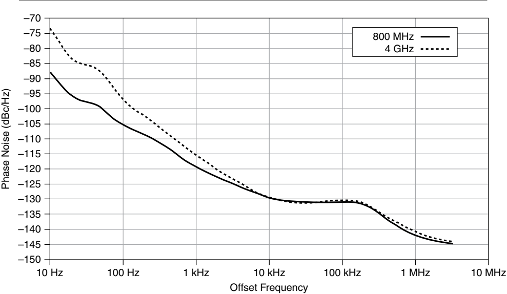
Figure 1. PXIe-5667 (7 GHz) Phase Noise at 800 MHz and 4 GHz Center Frequency (Nominal)
