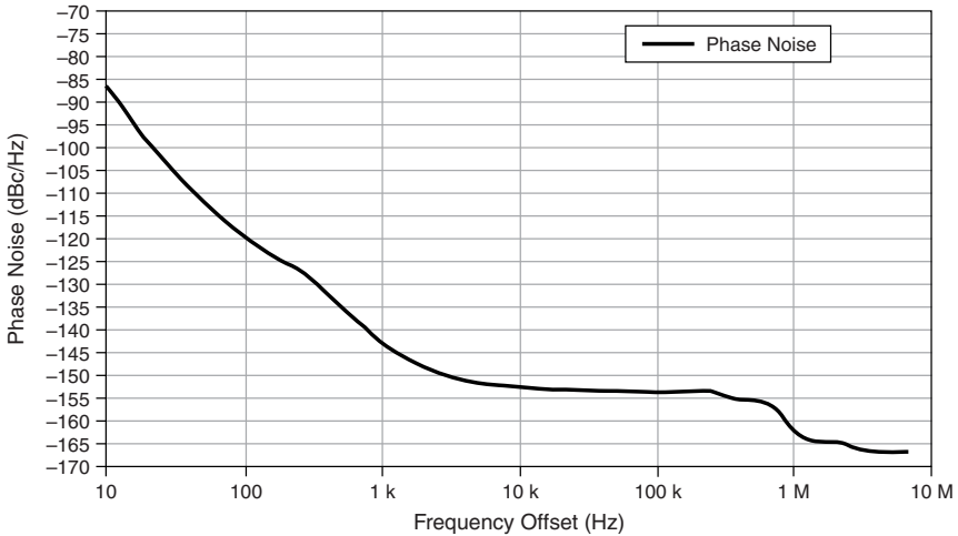
Figure 15. LO3 Phase Noise 45
