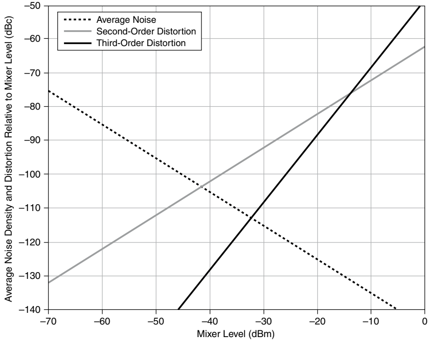
Figure 7. PX1e-5605 Downconverter Nominal Dynamic Range for Frequencies 3.6 GHz to 7.5 GHz, Preselector Present and Enabled (Nominal)
