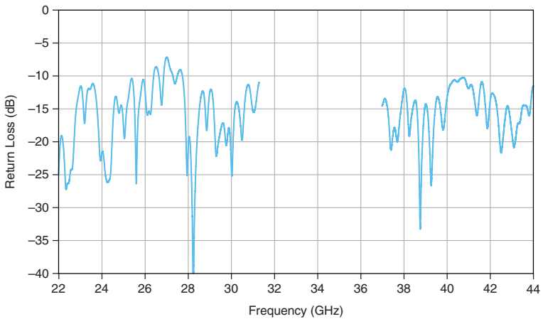
Figure 46. mmRH-5582 RF Output Port Return Loss, Measured at Switched TRX Port
