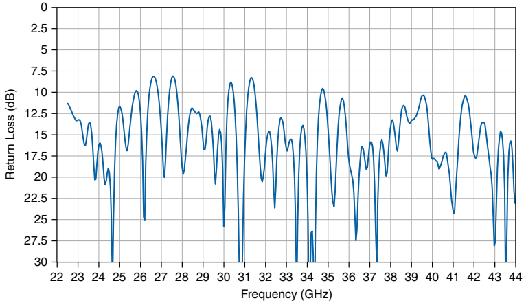
Figure 44. mmRH-5582 RF Output Port Return Loss, Measured at Direct TRX Port
