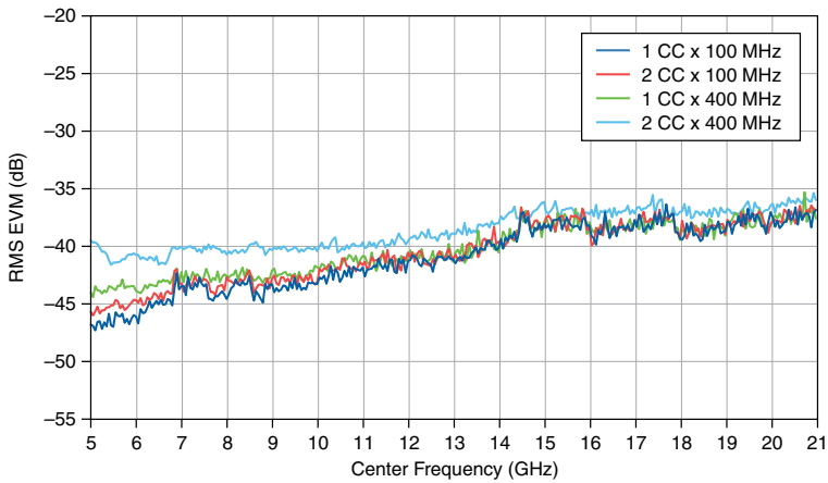
Figure 35. IF 5G NR RMS EVM versus Frequency (Independent LO2), Measured 26,31,32
