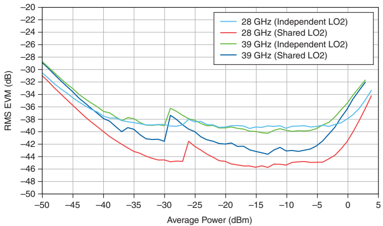
Figure 37. Switched to Switched RF 5G NR 1 CC x 100 MHz RMS EVM versus Average Power, Measured 33,34
