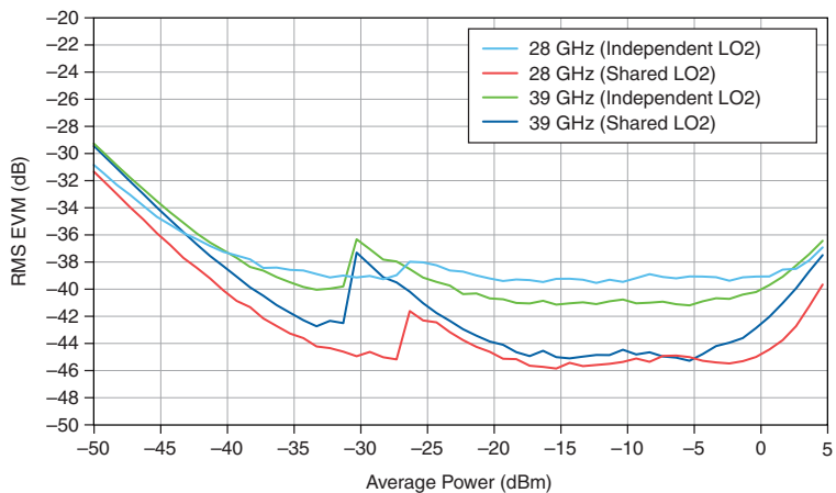
Figure 39. Direct TRX to Switched RF 5G NR 1 CC x 100 MHz RMS EVM versus Average Power, Measured 33,34
