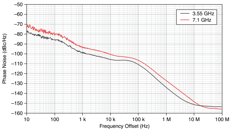
Figure 48. PXIe-3622 Internal LO1 VCO Phase Noise, Measured 42 (Spurs Not Shown)
