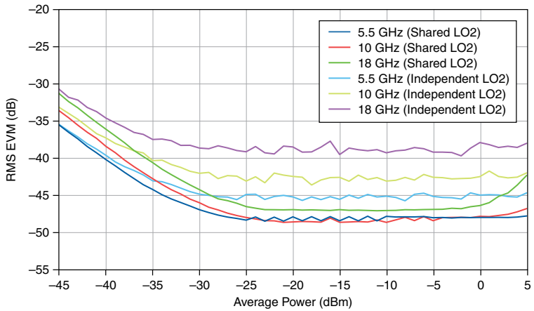
Figure 31. IF 5G NR 2 CC x 100 MHz RMS EVM versus Average Power, Measured 26,28
