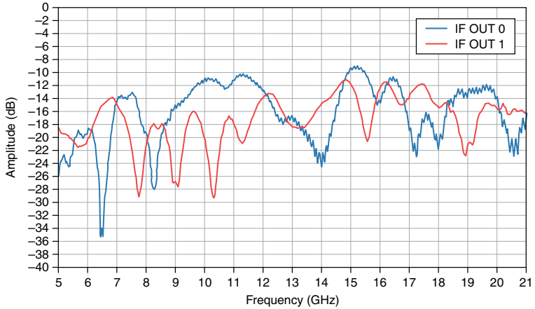
Figure 42. PXle-3622 IF OUT Port Return Loss, Measured
