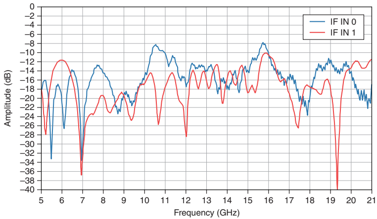
Figure 41. PXIe-3622 IF IN Port Return Loss, Measured
