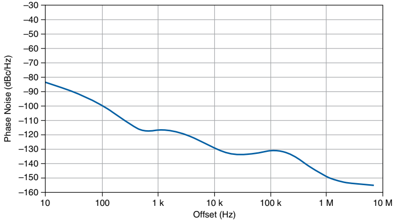
Figure 47. PXIe-5653 Phase Noise, Measured 41 (Spurs Not Shown)
