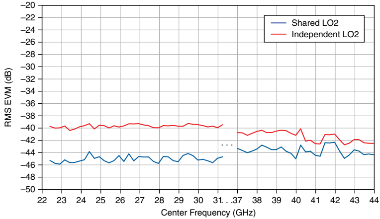
Figure 40. Direct TRX to Direct TRX RF 5G NR RMS EVM versus Frequency, Measured 33,34,35
