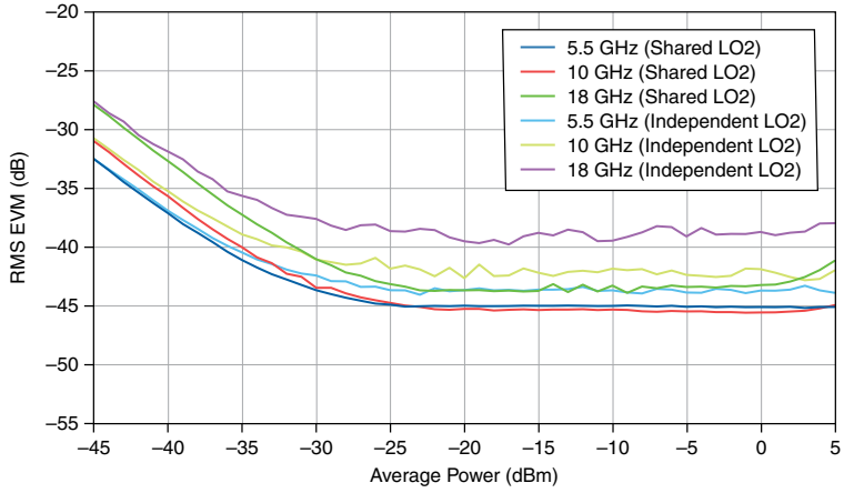
Figure 33. IF 5G NR 2 CC x 400 MHz RMS EVM versus Average Power, Measured 26,30
