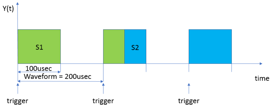
Figure 31. Graph of Burst Waveform with Triggers
