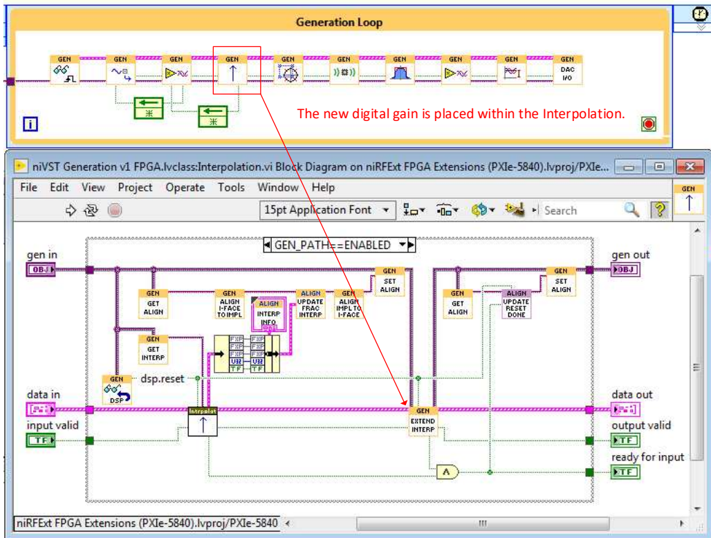
Figure 15. VSG Data Path with New Digital Gain
