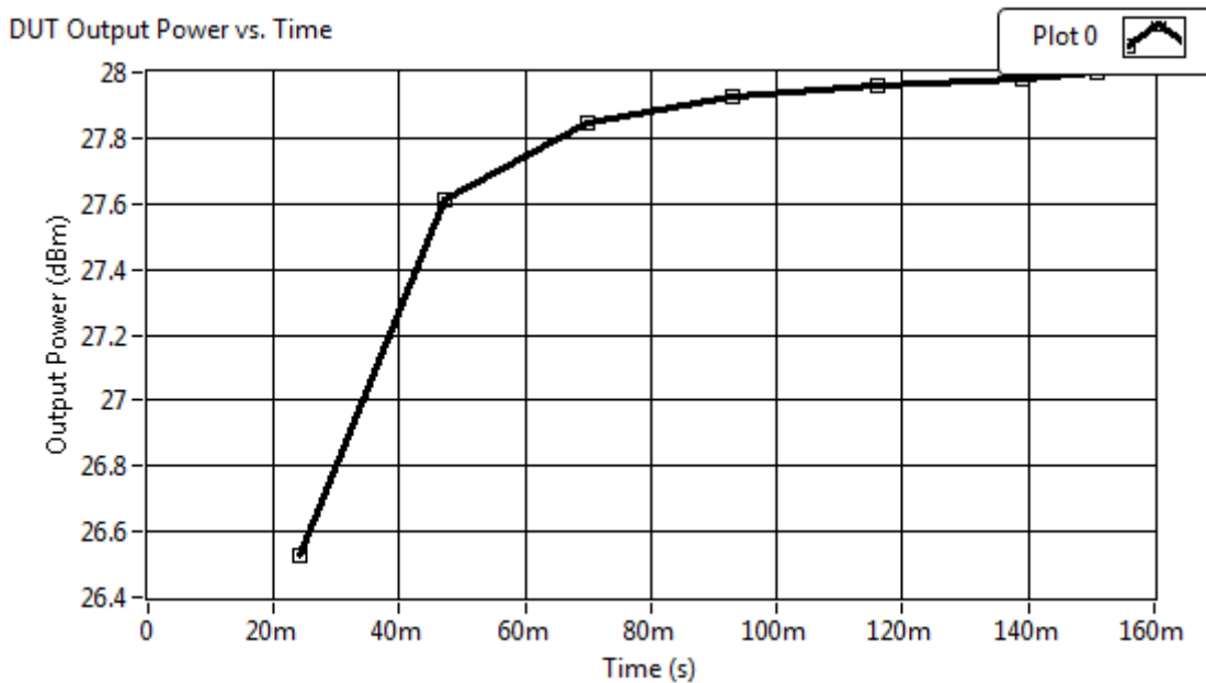
Figure 2. Graph of Traditional Leveling
