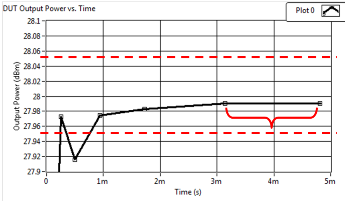
Figure 9. Limits for Determining the DUT is Leveled
