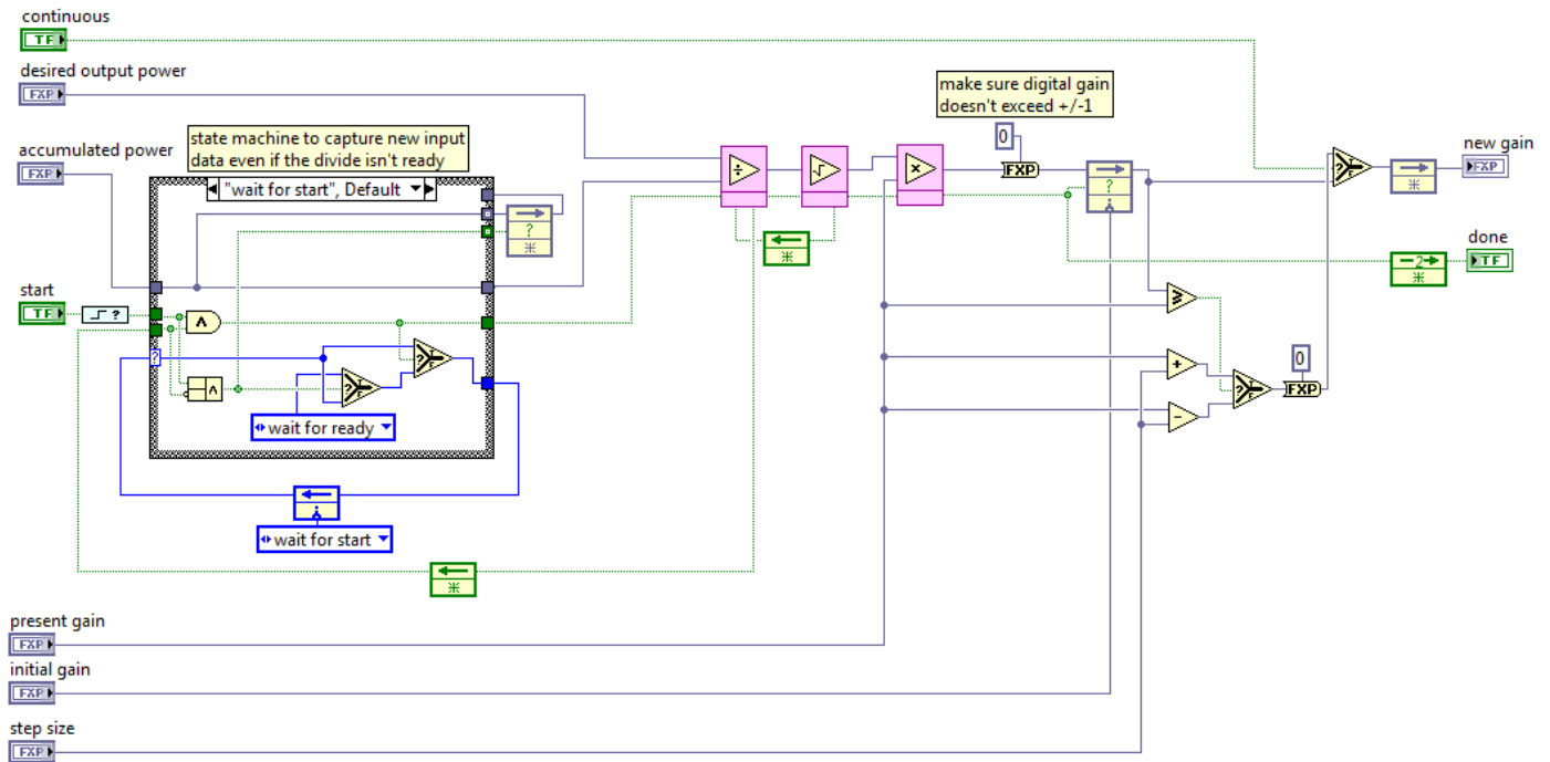
Figure 19. Calculate Gain Block Diagram
