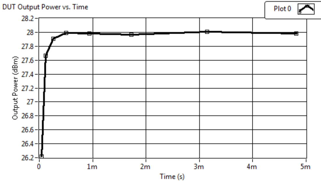
Figure 8. Graph of Hardware-Based Leveling
