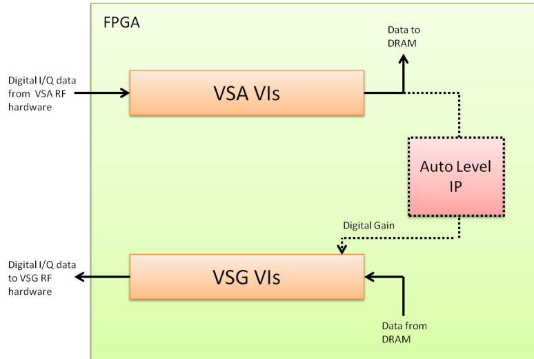
Figure 4. VST with Auto Level IP
