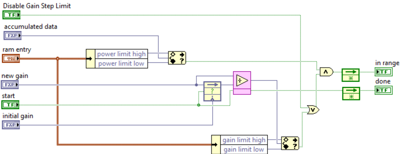
Figure 20. In Range Block Diagram
