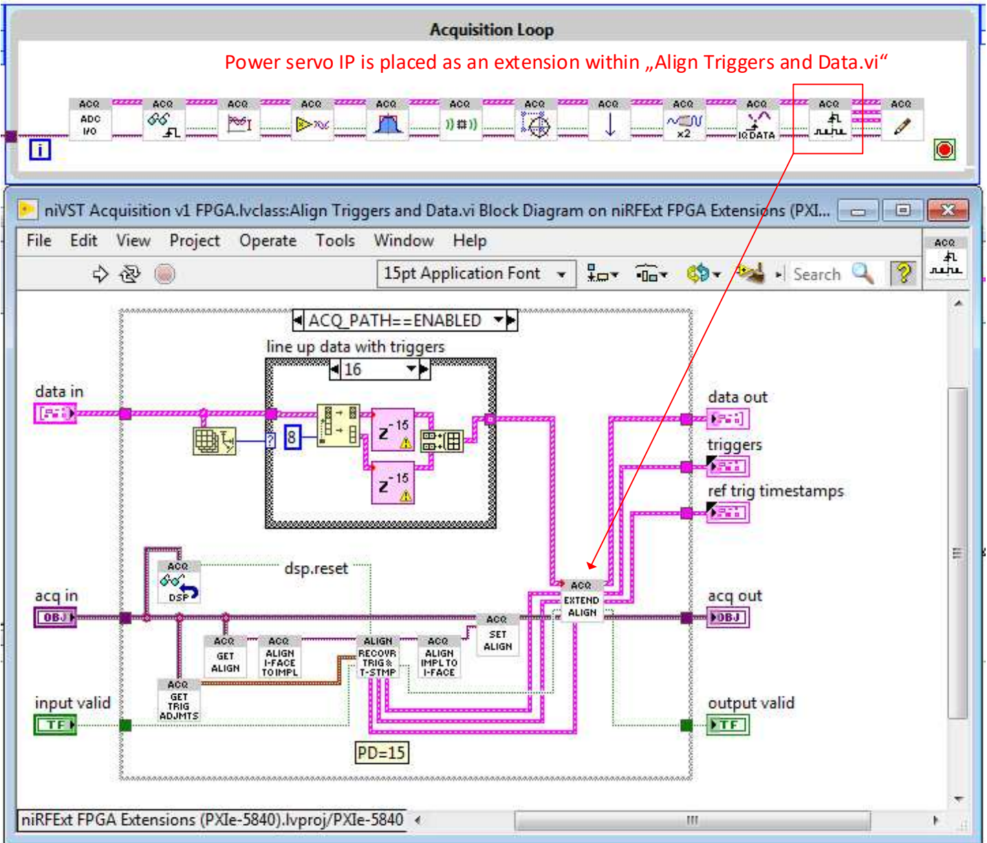
Figure 14. VSA Data Path
