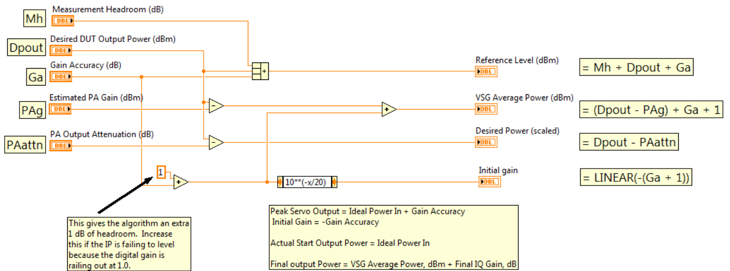
Figure 23. Calculate Servo Parameters Block Diagram
