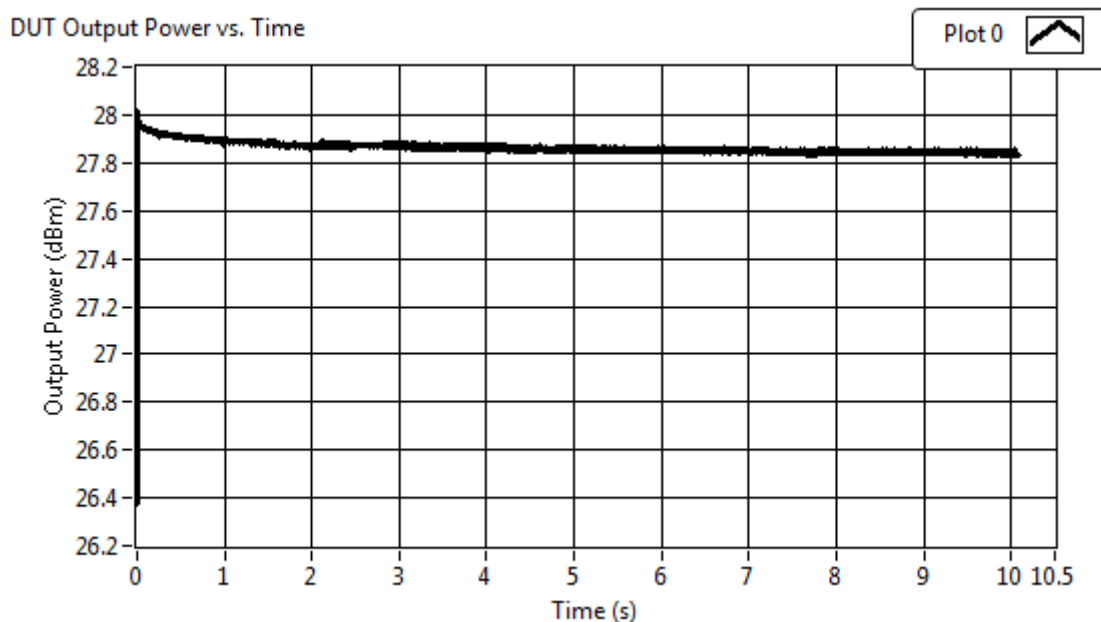
Figure 11. Thermal Droop with Hardware-Based Leveling
