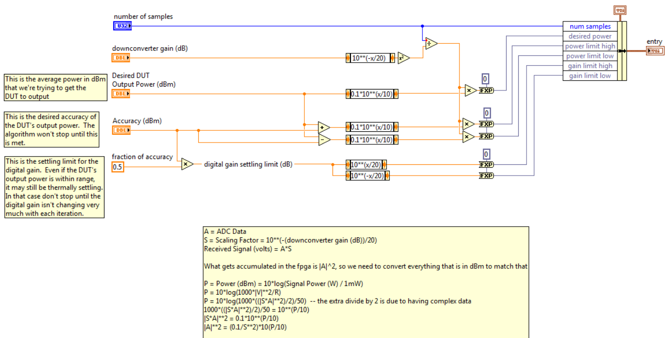
Figure 24. Build Averaging Schedule Entry Block Diagram
