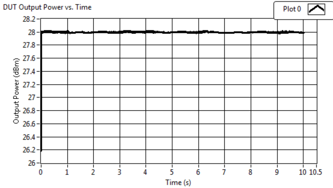
Figure 13. Continuous Hardware-Based Leveling
