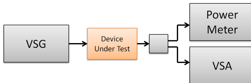
Figure 1. Traditional PA Test Setup
