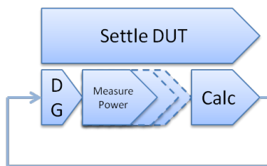
Figure 7. Leveling Loop with Averaging Schedule
