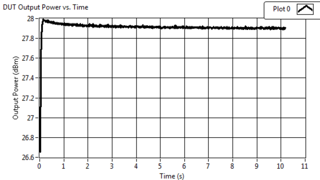
Figure 10. Thermal Droop with Traditional Leveling
