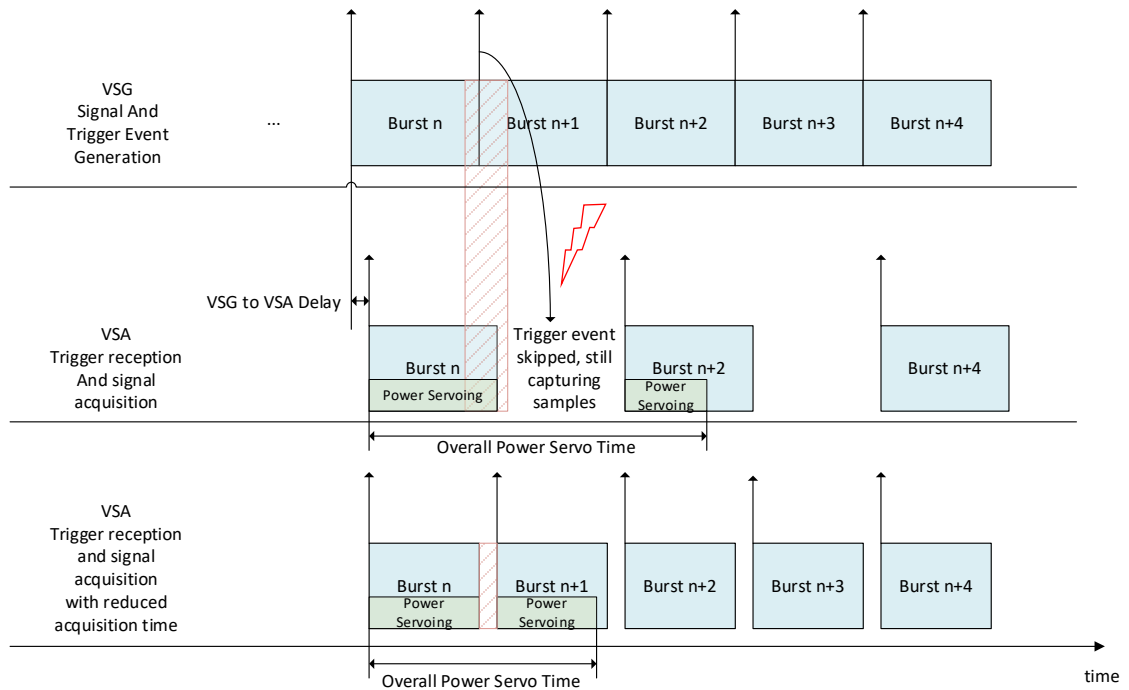
Figure 32. Active Window Config Case 1
