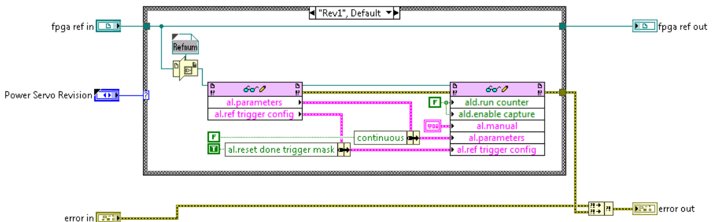
Figure 28. Reset Block Diagram
