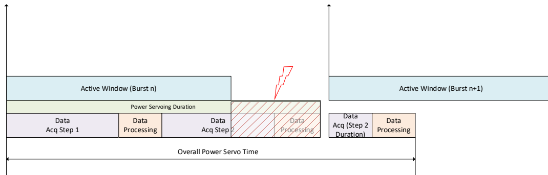
Figure 33. Active Window Config Case 2
