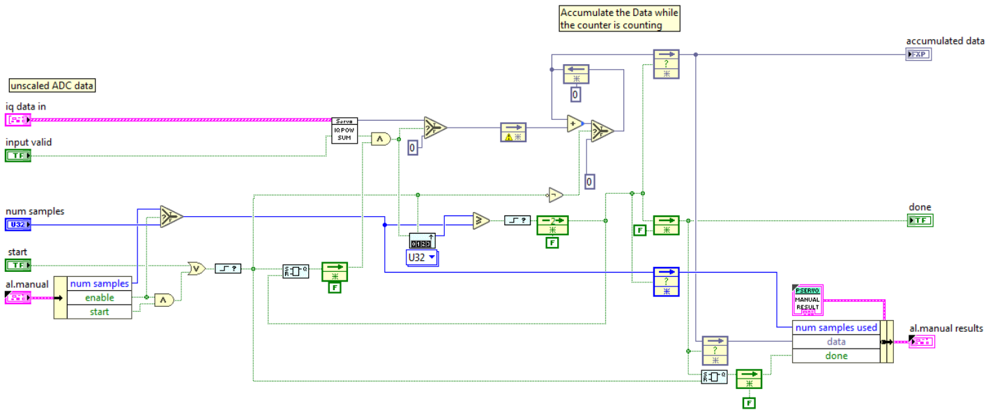
Figure 18. Accumulate IQ Data Block Diagram
