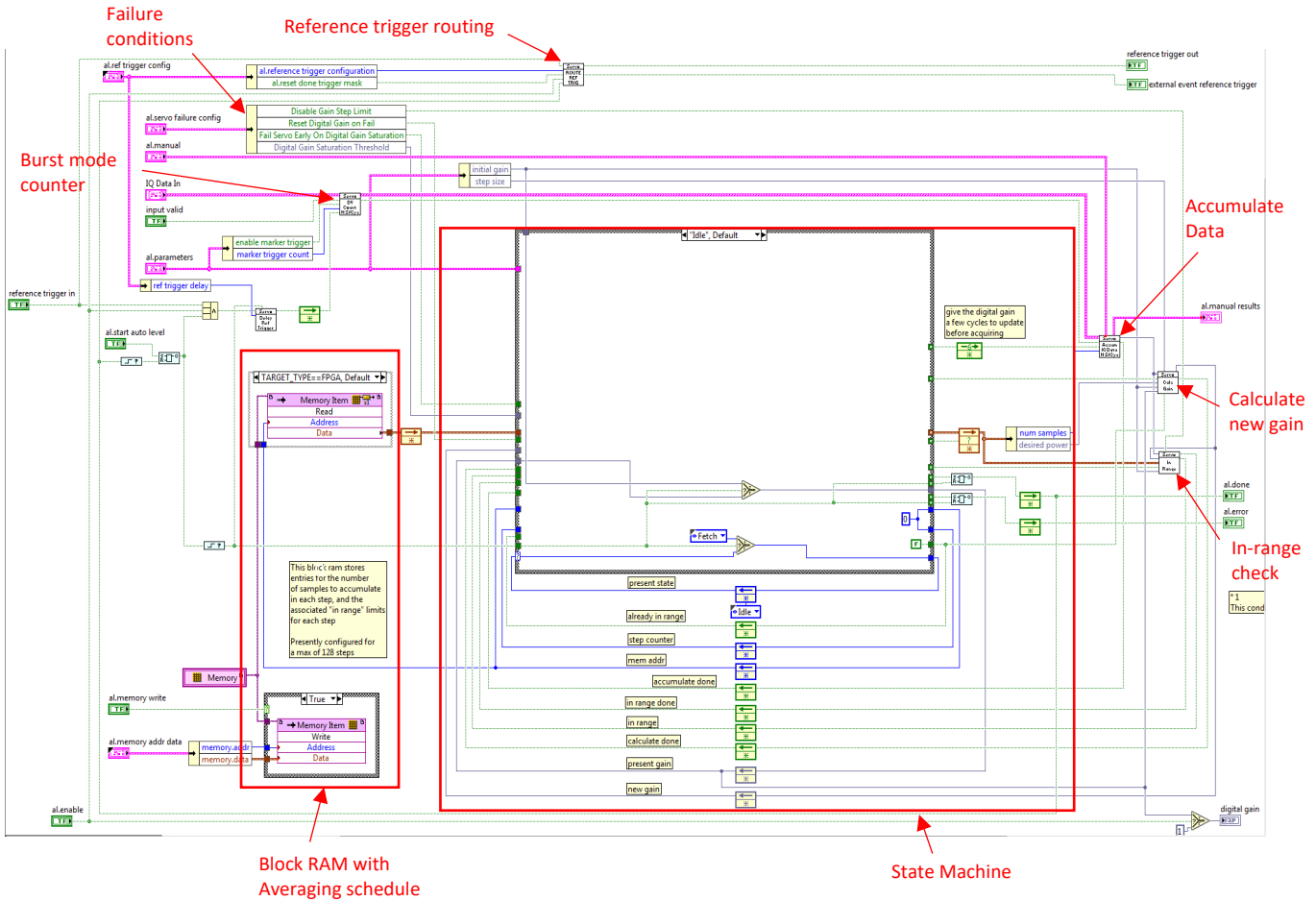
Figure 16. Auto Level VI Block Diagram
