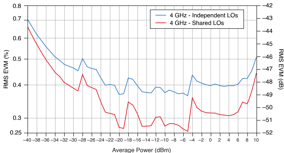
Figure 31. 5G NR Measured RMS EVM (dB and %) Versus Measured Average Power (dBm)
