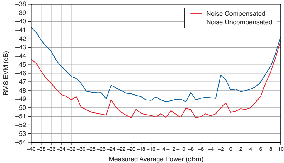
Figure 26. WLAN 802.11ax Measured RMS EVM (dB) Versus Measured Average Power (dBm)
