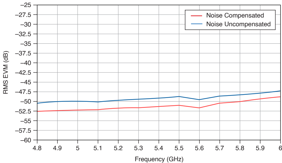
Figure 25. WLAN 802.11ax Measured RMS EVM (dB) Versus Frequency (Hz)
