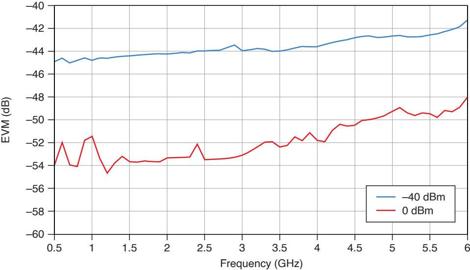
Figure 22. Measured RMS EVM
