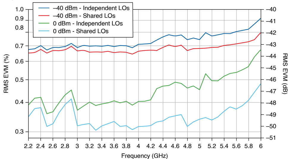
Figure 30. 5G NR Measured RMS EVM (dB and %) Versus Frequency (Hz)
