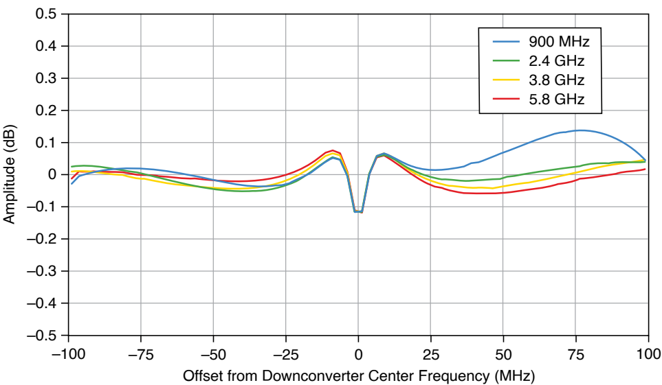
Figure 4. Measured 200 MHz Input Frequency Response, 0 dBm Reference Level, Normalized to 3.75 MHz
