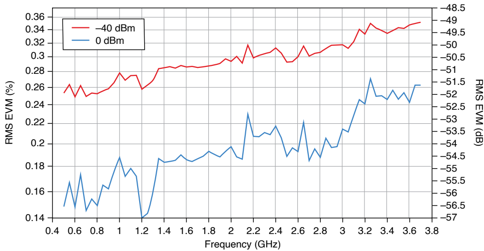
Figure 32. LTE Measured RMS EVM (dB and %) Versus Frequency (Hz)
