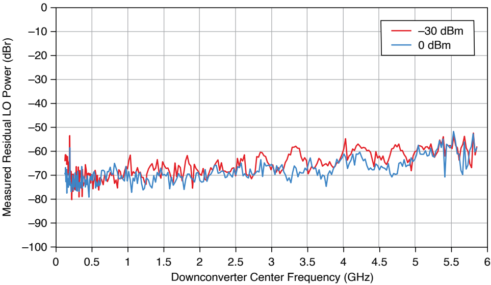
Figure 8. Input LO Residual Power, Measured (PXIe-5841)
