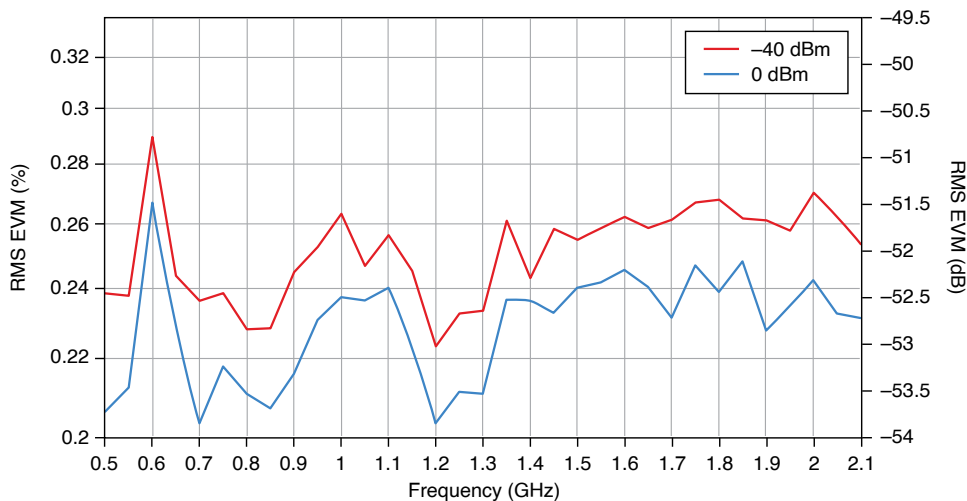
Figure 33. WCDMA Measured RMS EVM (dB and Percent) Versus Frequency (Hz)
