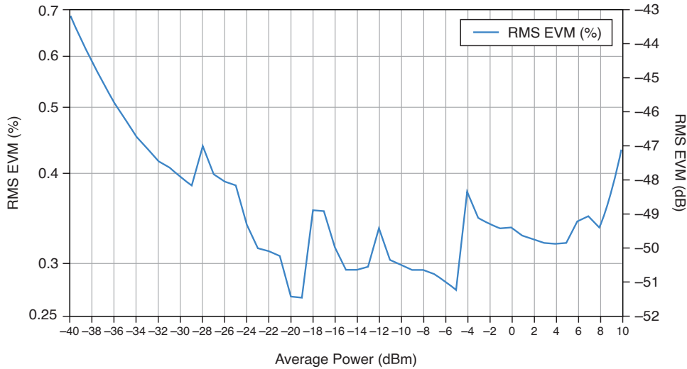
Figure 24. 5G NR Measured RMS EVM (dB and %) Versus Measured Average Power (dBm)
