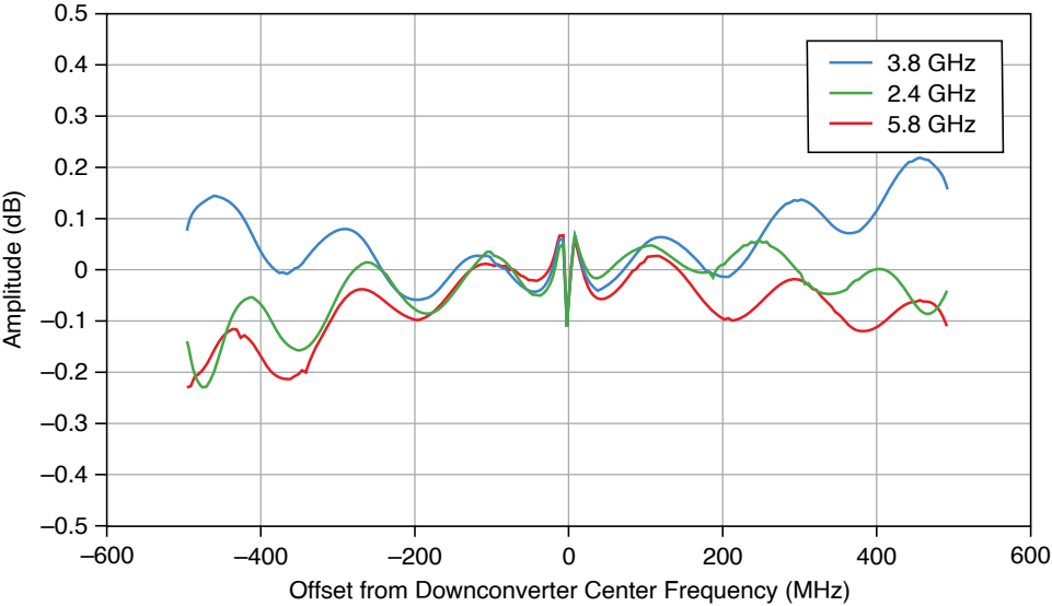
Figure 5. Measured 1 GHz Input Frequency Response, 0 dBm Reference Level, Normalized to 3.75 MHz
