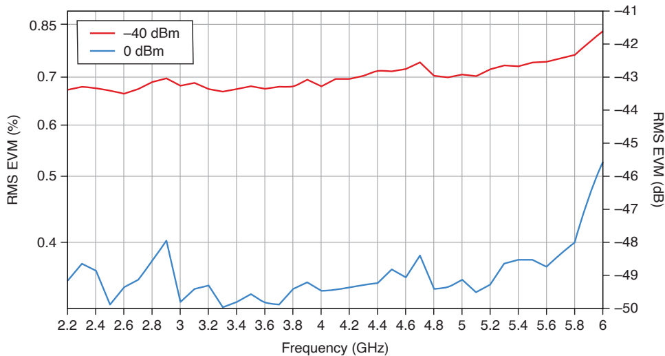
Figure 23. 5G NR Measured RMS EVM (dB and %) Versus Frequency (Hz)
