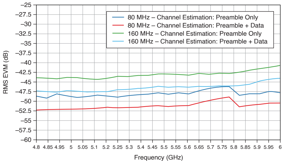
Figure 27. WLAN 802.11ac Measured RMS EVM (dB) Versus Frequency (Hz)
