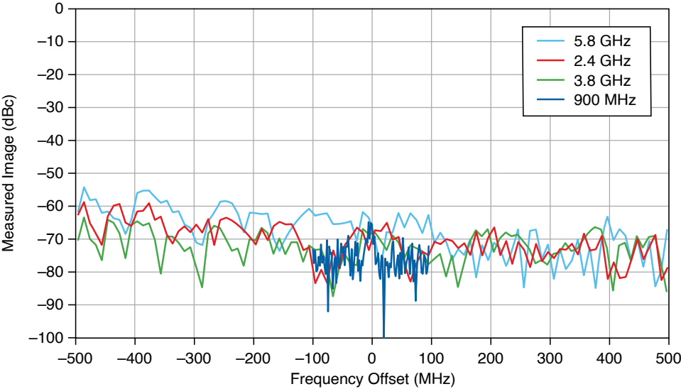
Figure 11. Input Residual Sideband Image, -30 dBm Reference Level, Measured
