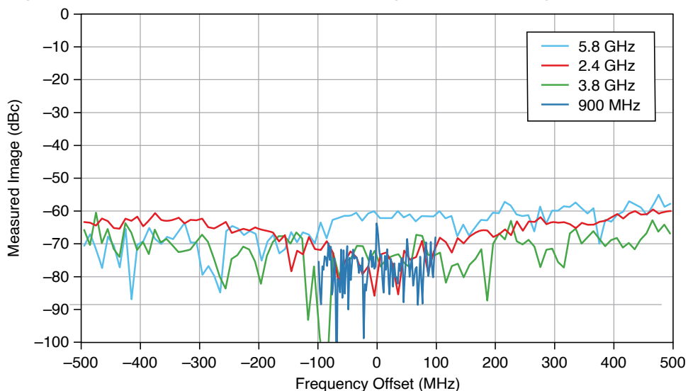
Figure 20. Output Residual Sideband Image, 0 dBm Average Output Power, Measured
