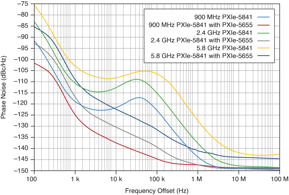
Figure 2. Measured Phase Noise for PXIe-5841 and PXIe-5655
