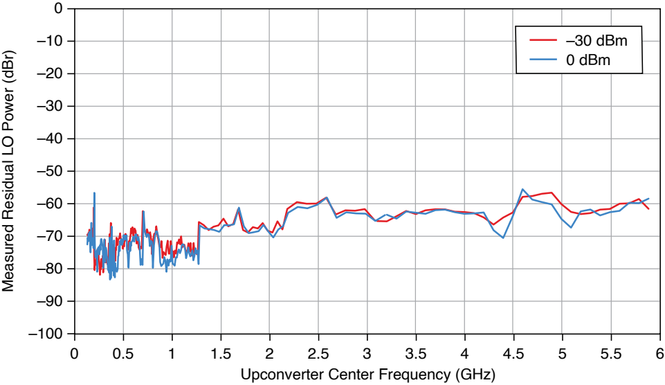
Figure 18. Output LO Residual Power, Measured (PXIe-5841)
