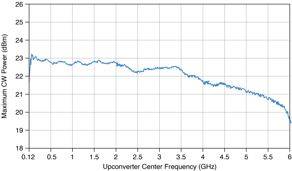
Figure 12. Output Maximum CW Average Power (dBm), Measured
