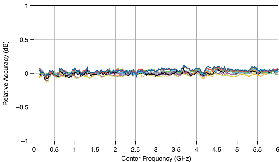
Figure 13. Output Relative Power Accuracy, 120 MHz to 6 GHz, -65 dBm to +15 dBm, Normalized to 0 dBm Power Level, Measured
