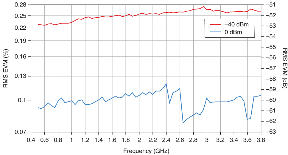
Figure 28. LTE Measured RMS EVM (dB and %) Versus Frequency (Hz)
