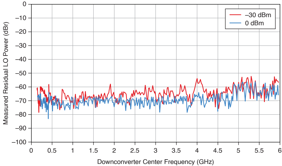
Figure 9. Input LO Residual Power, Measured (PXle-5841 with PXle-5655)
