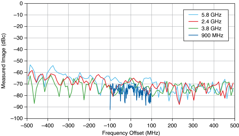
Figure 10. Input Residual Sideband Image, 0 dBm Reference Level, Measured
