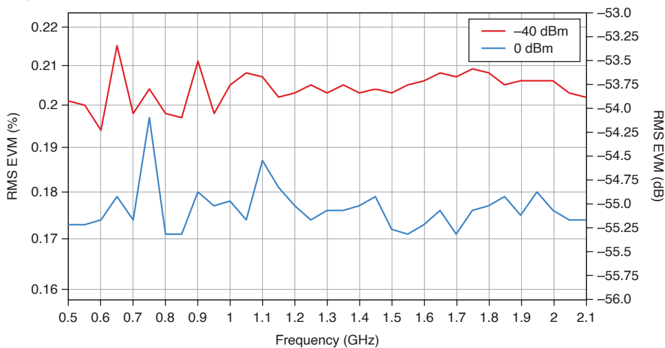
Figure 29. WCDMA Measured RMS EVM (dB and %) Versus Frequency (Hz)
