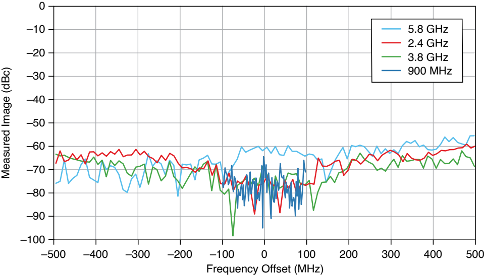
Figure 21. Output Residual Sideband Image, -30 dBm Average Output Power, Measured
