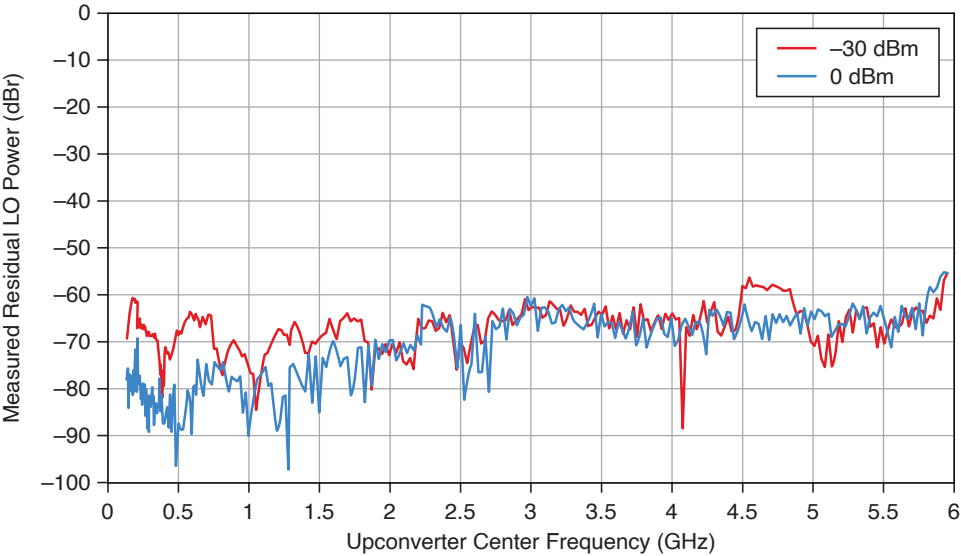
Figure 19. Output LO Residual Power, Measured (PXIe-5841 with PXIe-5655)
