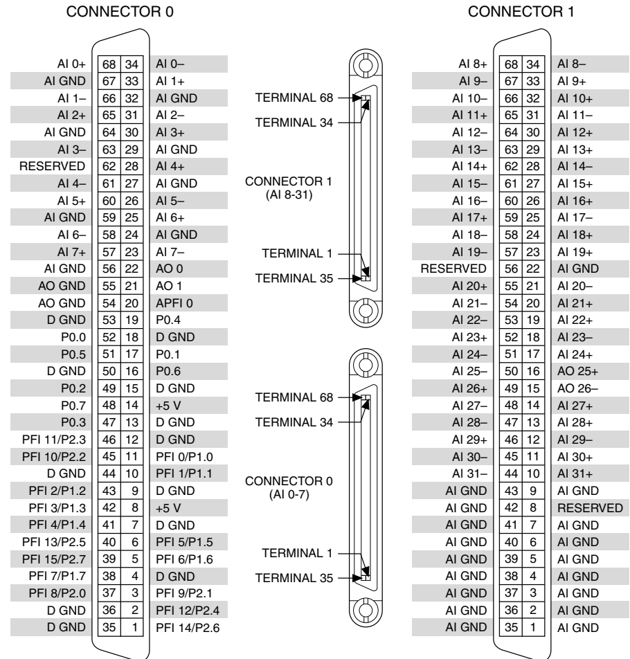
Figure 5. PXIe-6349 Pinout
