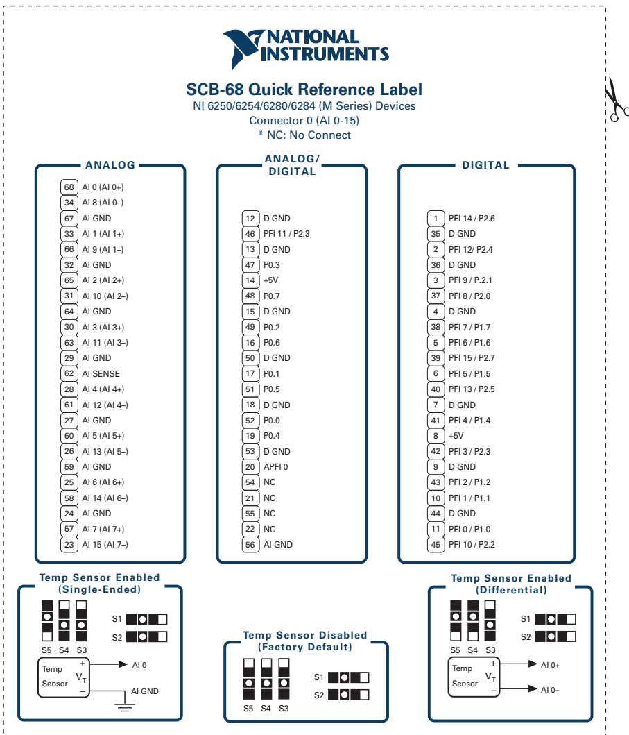
Figure 3. NI 6250/6254/6280/6284 Connector 0
