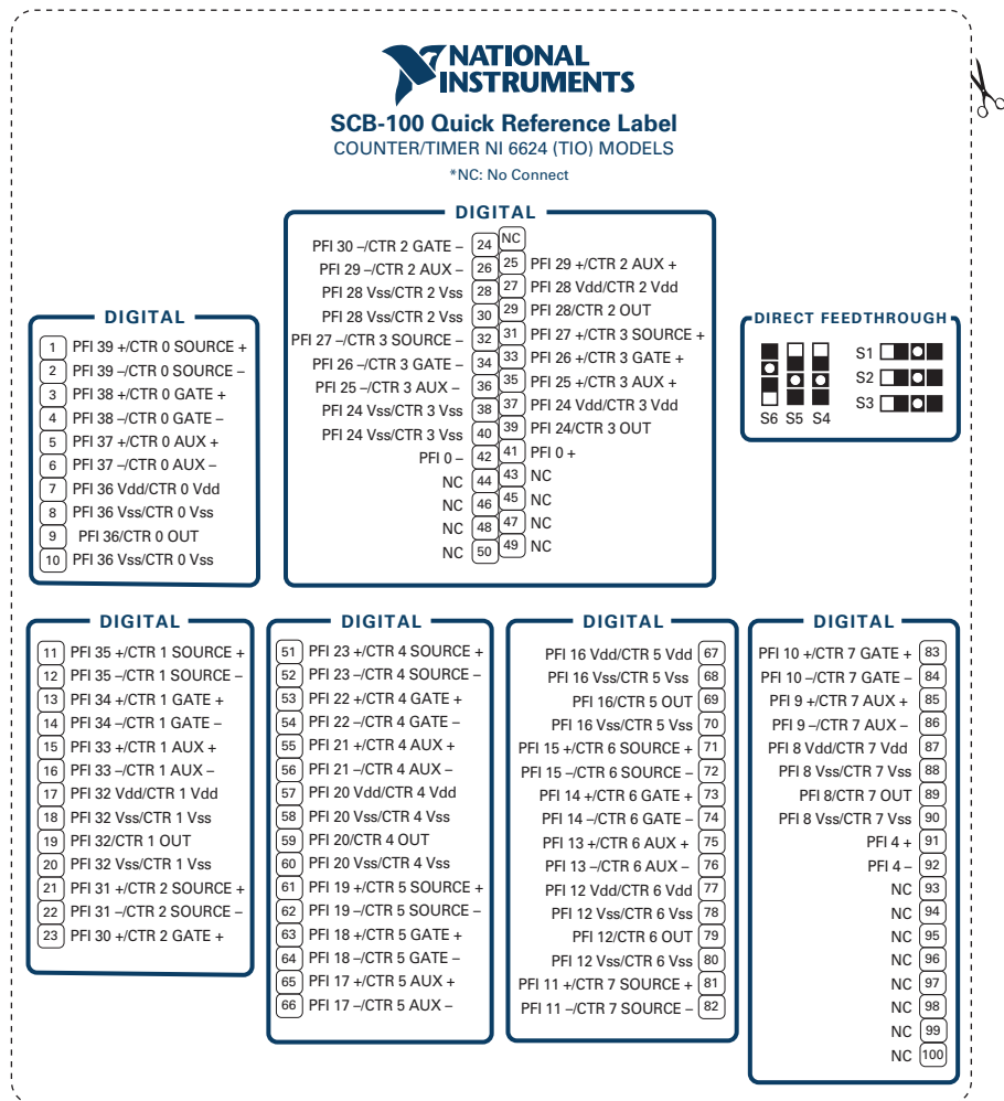
Figure 1. NI 6624
