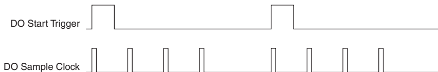
Figure 5-8. Retriggerable DO
