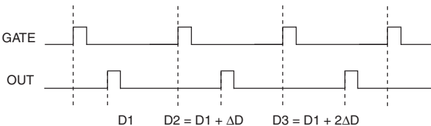
Figure 6-36. Pulse Generation for ETS
