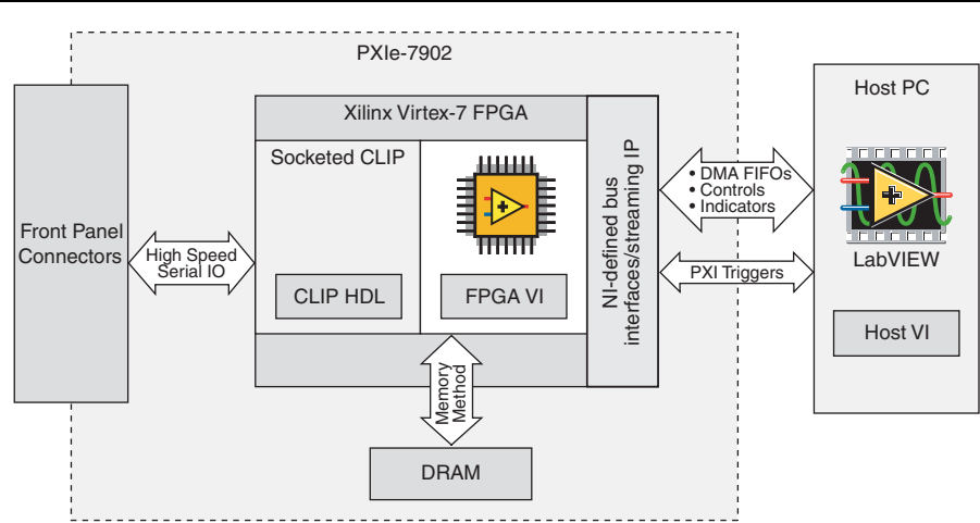
Figure 6-1. PXIe-7902 System Architecture Elements
