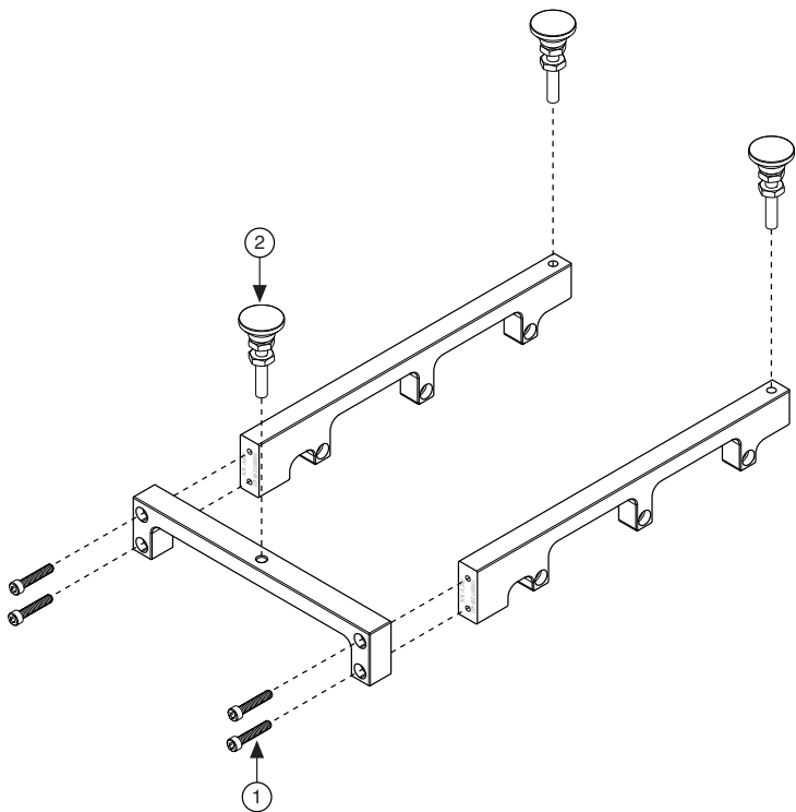
Figure 1. Assembling the Tripod
