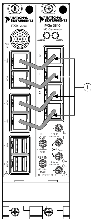
Figure 24. Interconnecting the PXIe-7902 and PXIe-3610 Modules
