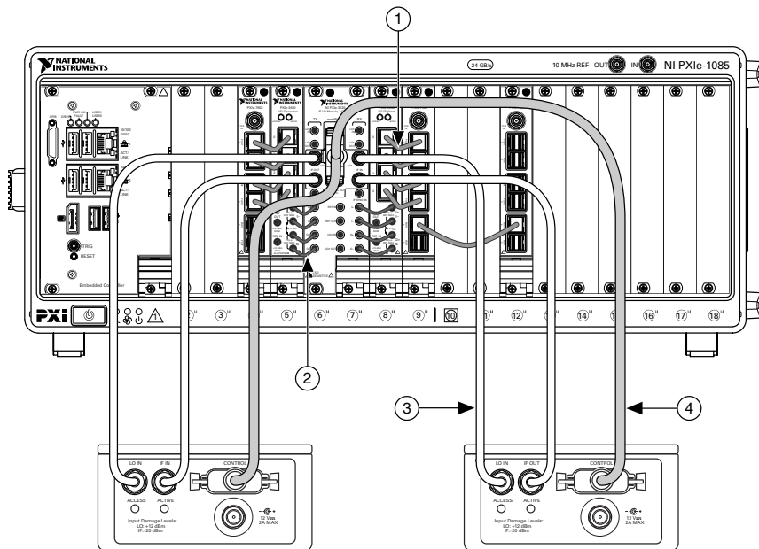
Figure 35. Connecting mmWave Heads to the Bidirectional SISO (Baseband and IF) System
