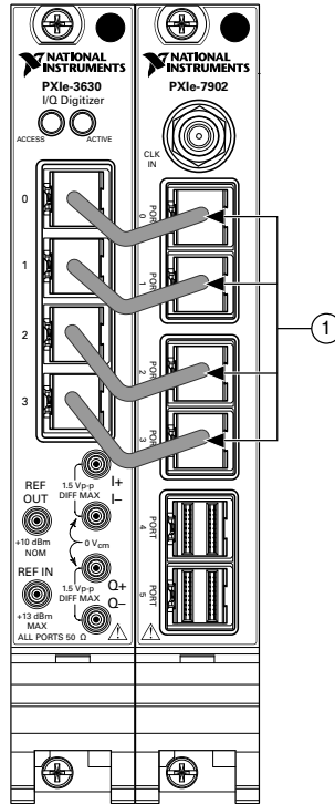
Figure 12. Interconnecting the PXIe-3630 and PXIe-7902 Modules
