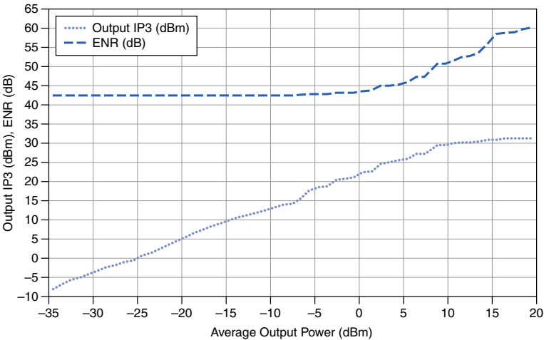
Figure 17. mmRH-3647 mmWave Radio Head Simulated Output IP3 and ENR 17
