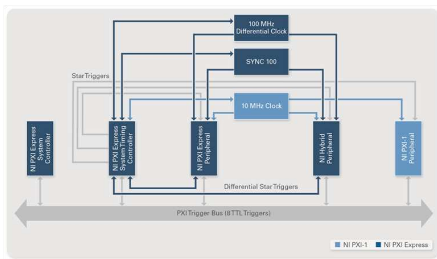
Figure 5. PXI High-Speed Serial Instruments lock to the 100MHz differential clock to stay aligned with other instrumentation in the PXI chassis and have access to PXI triggers to align acquisition or generation.
