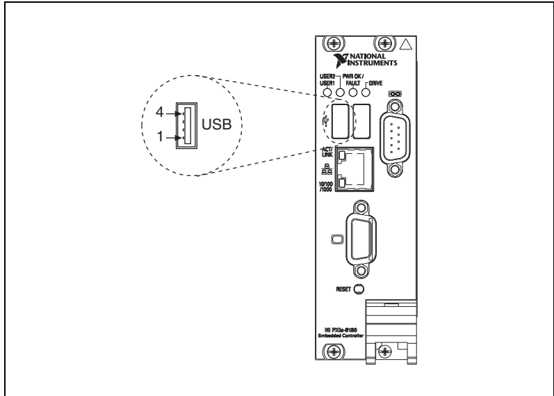
Figure 3-5. USB Connector Location and Pinout
