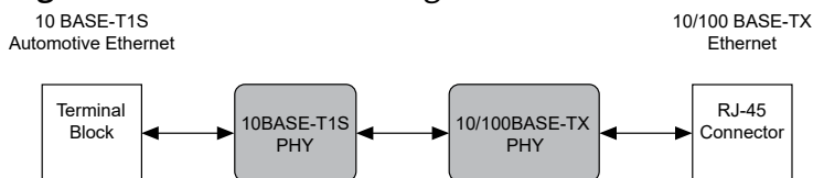
Figure 2. IVN-8563 Block Diagram
