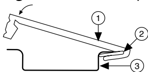
Figure 5. DIN Rail Clip Parts
