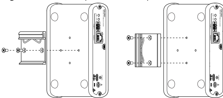
Figure 1. DIN Rail Clip Installation Options
