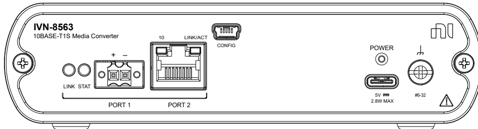
Figure 3. IVN-8563 Front Panel
