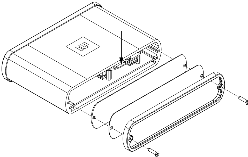
Figure 1. Removing the Rear Panel
