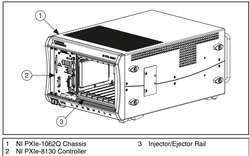
Figure 2. NI PXIe-8130 Controller Installed in a PXI Express Chassis
