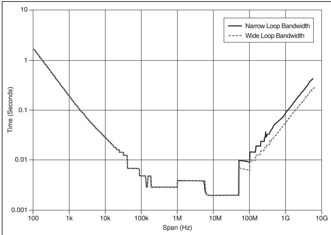
Figure 6. NI 5663 Measurement Time
