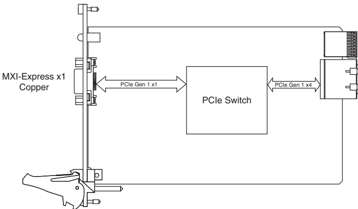
Figure 1-10. NI PXIe-8364 (193970x-01L) Block Diagram
