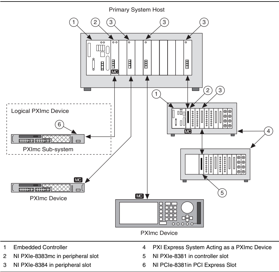
Figure 2. Example PXImc System
