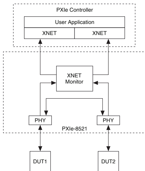
Figure 6. Tap Mode
