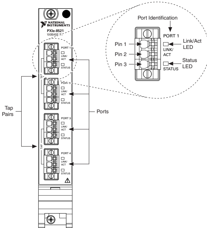
Figure 3. PXle-8521 Pinout
