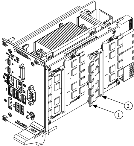
Figure 4. Installing a SO-DIMM in a PXIe-8881 Controller
