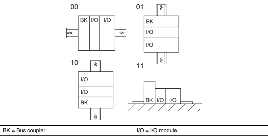
Figure 1. Mounting position
