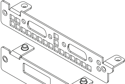
Figure 1. NI RMC-8355 Mounting Brackets
