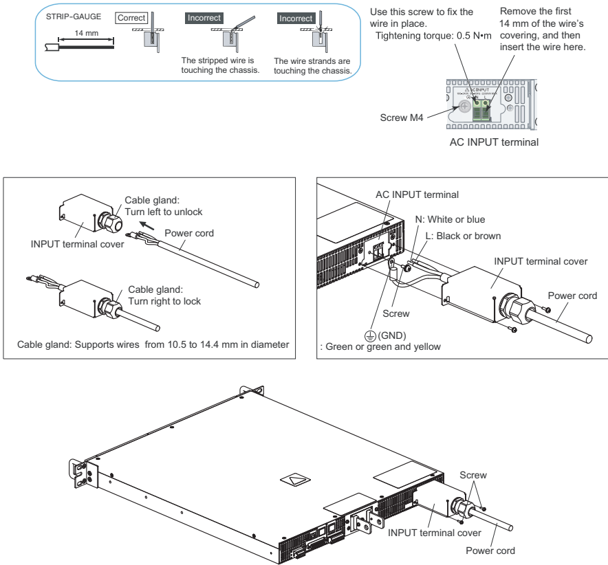
Figure 3. Connecting the Power Cord
