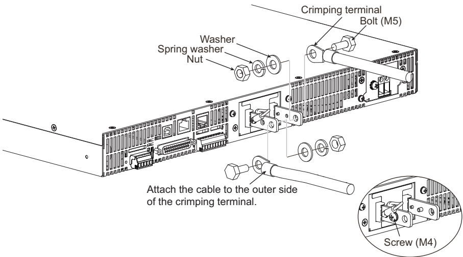
Figure 8. Connection Using M5 Bolt Set for RMX-4122/4123/4126/4127
