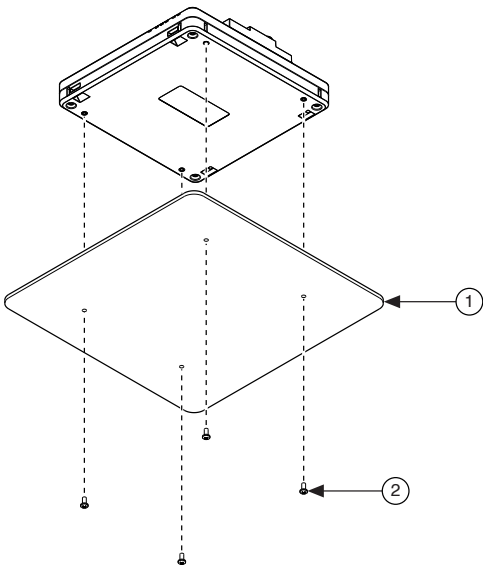
Figure 15. Mounting NI roboRIO 2.0 Using Screws
