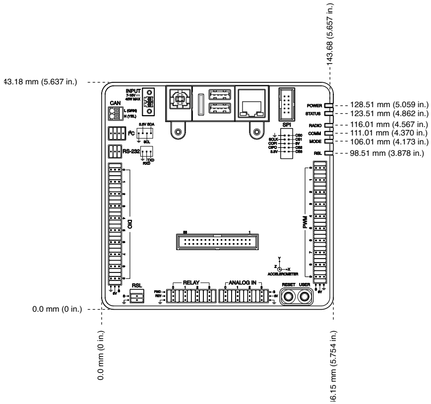
Figure 3. Dimensions, Primary Side LEDs
