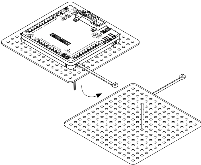
Figure 7. Step 2 to Secure One Edge of the Device
