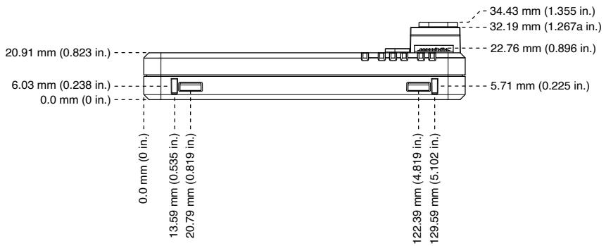
Figure 5. Dimensions, Side
