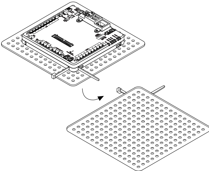
Figure 11. Step 2 to Secure One Corner of the Device
