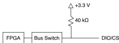
Figure 30. DIO Lines with 40 k \Omega Pullup Resistors to 3.3 V
