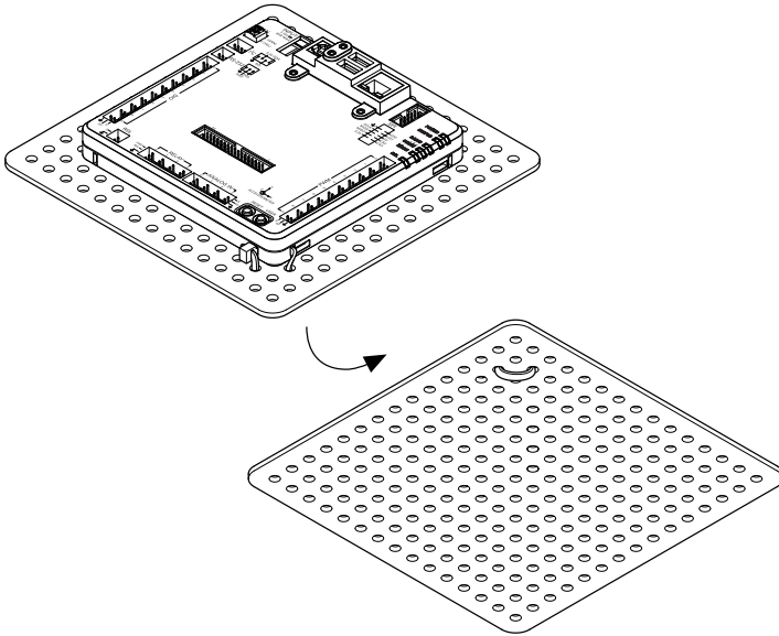
Figure 14. Step 5 to Secure One Corner of the Device
