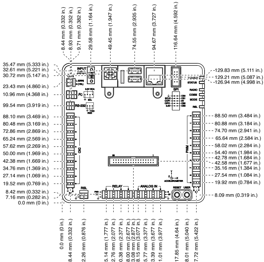
Figure 2. Dimensions, Primary Side
