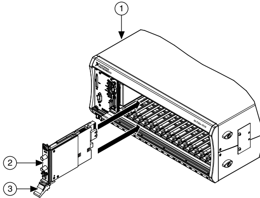
Figure 3. Module Installation
